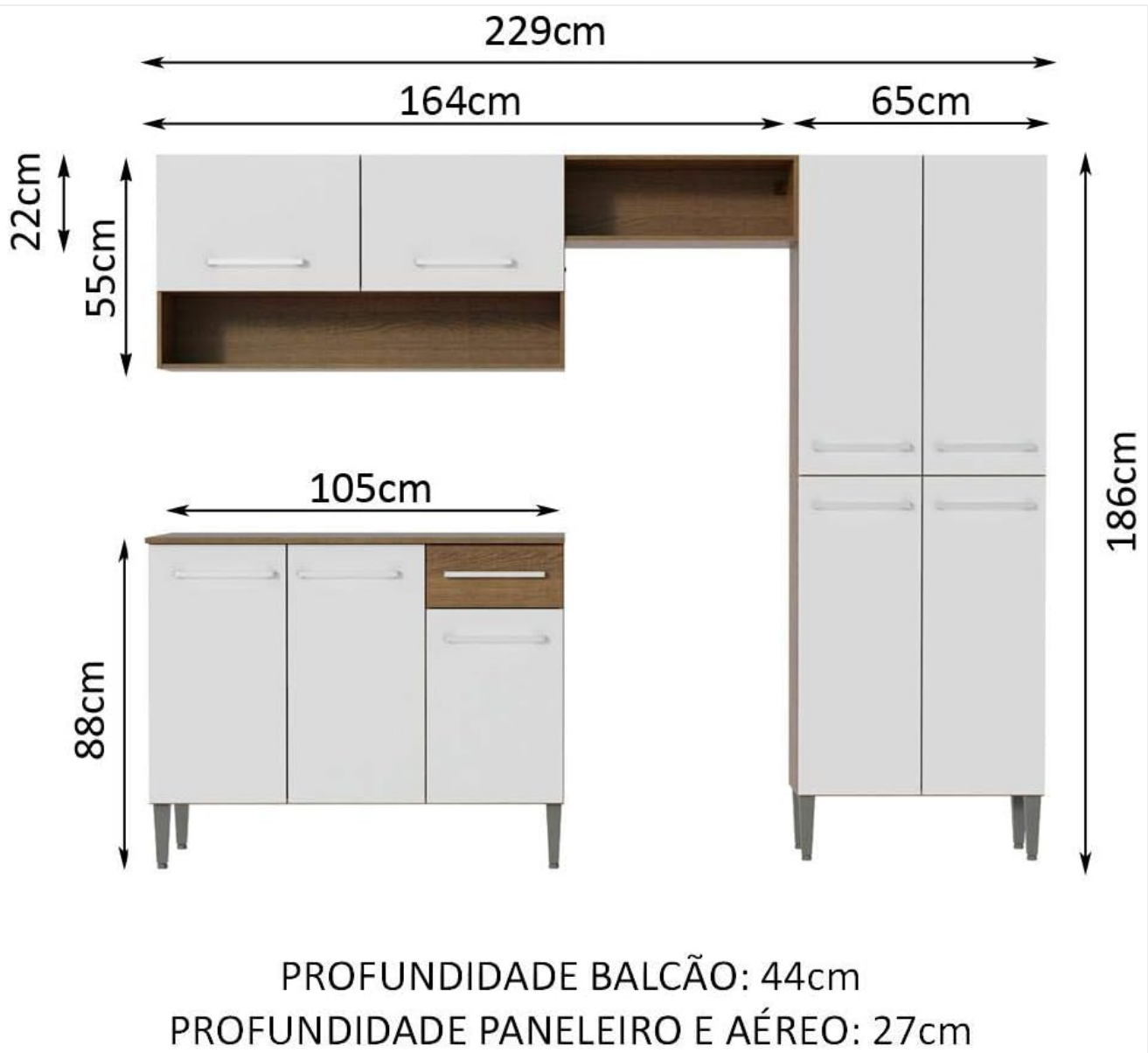
Image 3: Overall dimensions and individual component measurements for planning.
