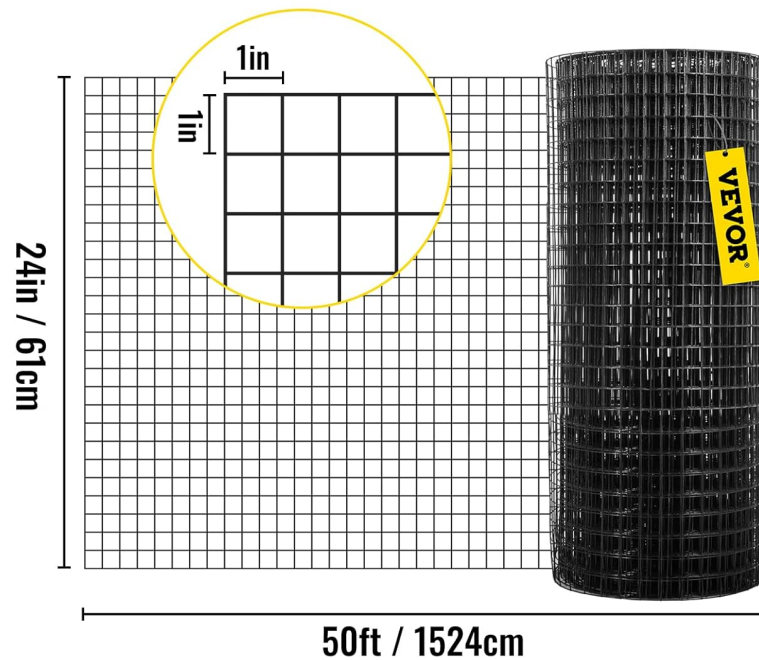
Figure 4.1: Product dimensions and mesh size.
