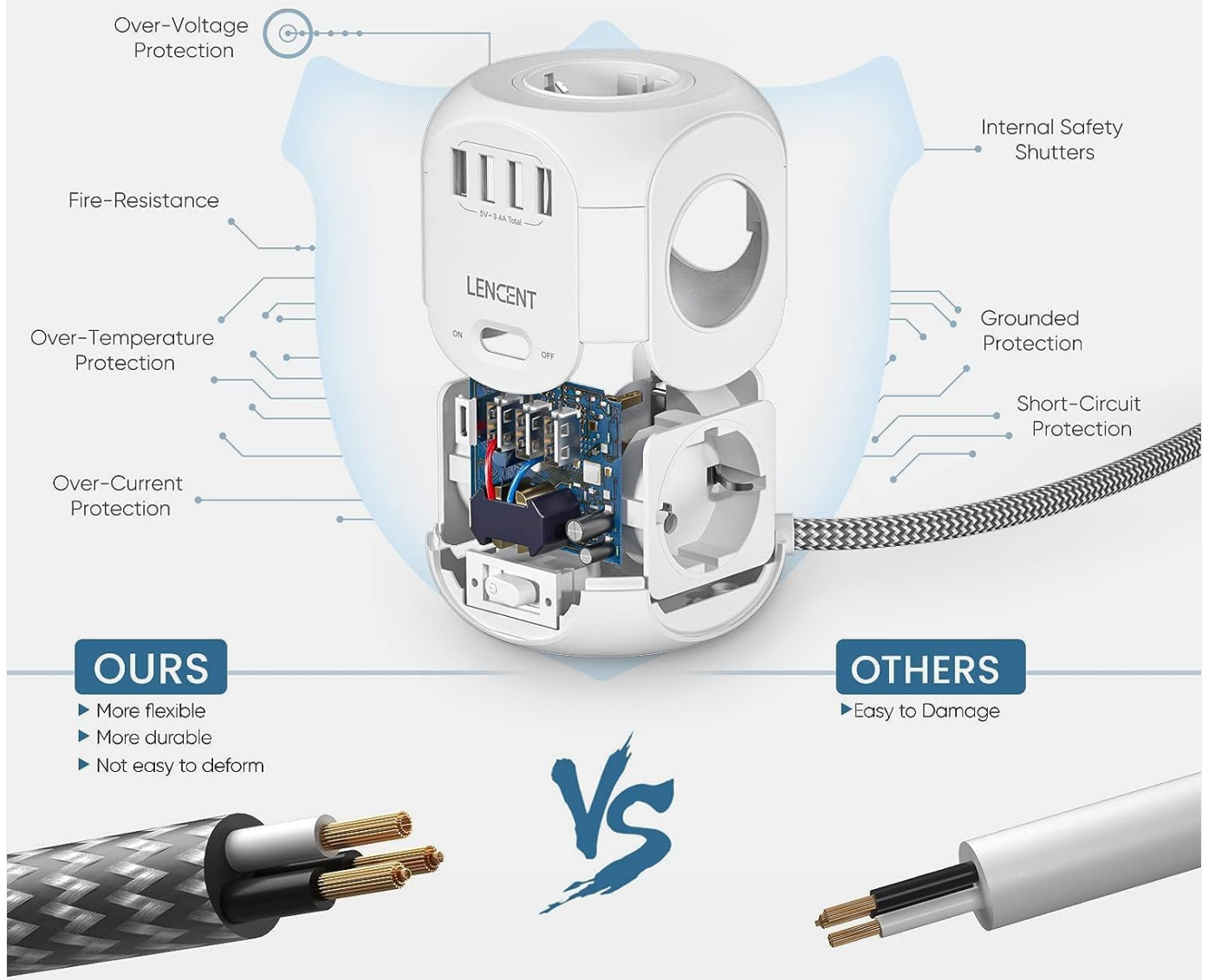
Figure 2: Illustration of the comprehensive safety features integrated into the power strip.
