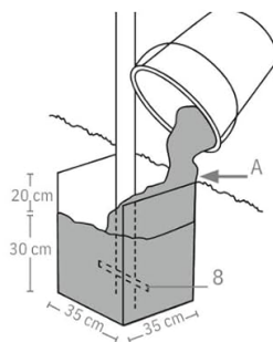
Figure 3.1: Visual guide for the 5-step installation process, emphasizing the concrete anchoring for a safe and stable construction.
