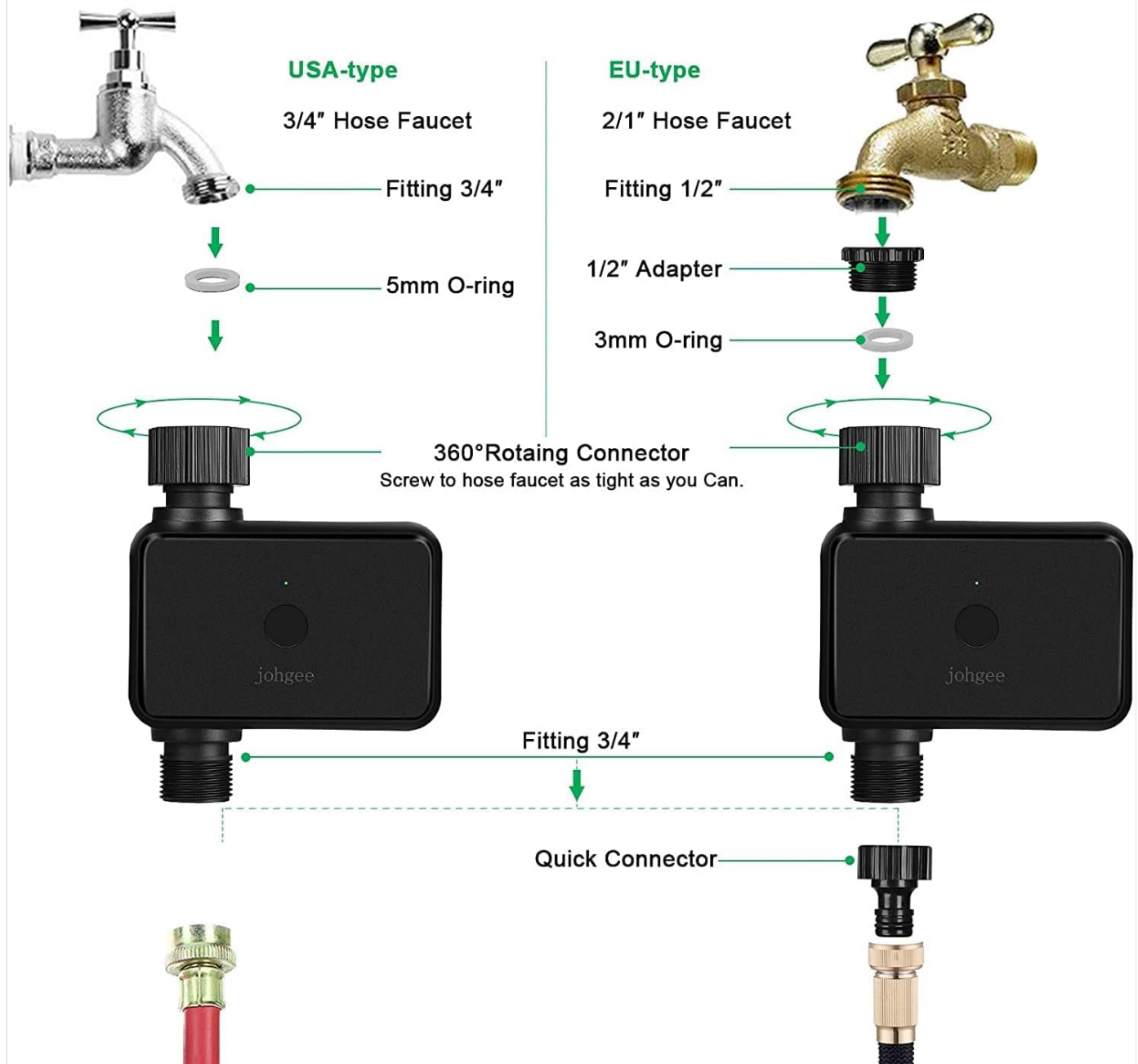
Image: A diagram illustrating how to connect the Johgee Smart Water Timer to different faucet types (USA and EU) using the provided adapters and O-rings. It also shows the 360-degree rotating connector for easy installation.
