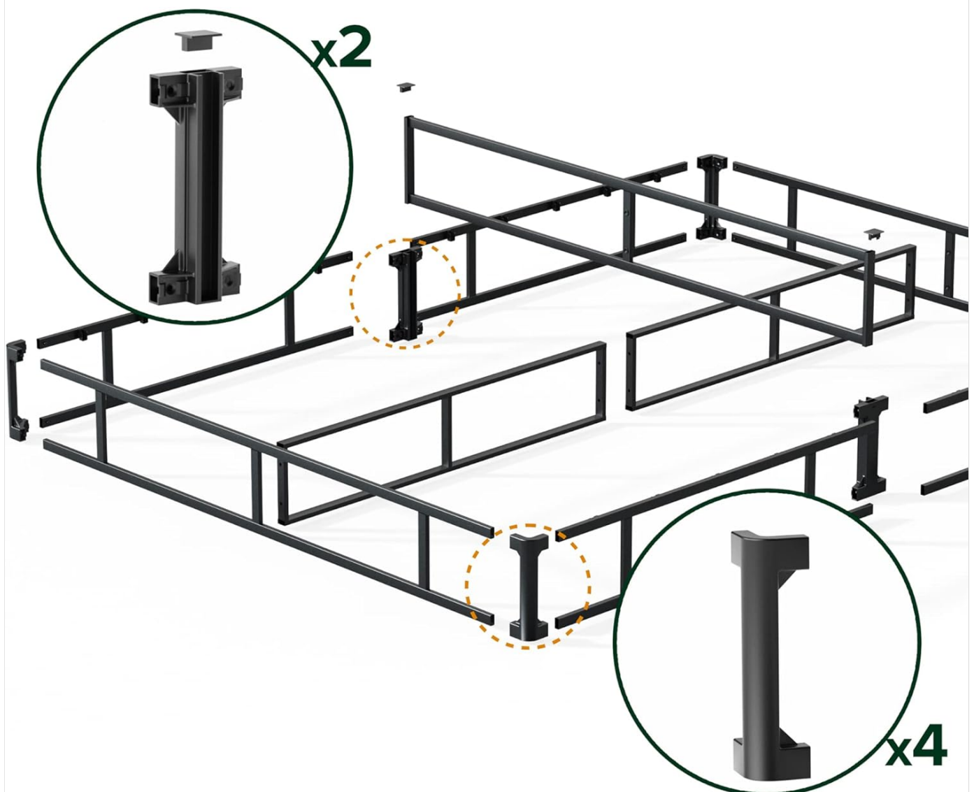
Image: Illustration demonstrating the tool-free locking brackets, which simplify the assembly process by reducing the need for traditional bolts.
