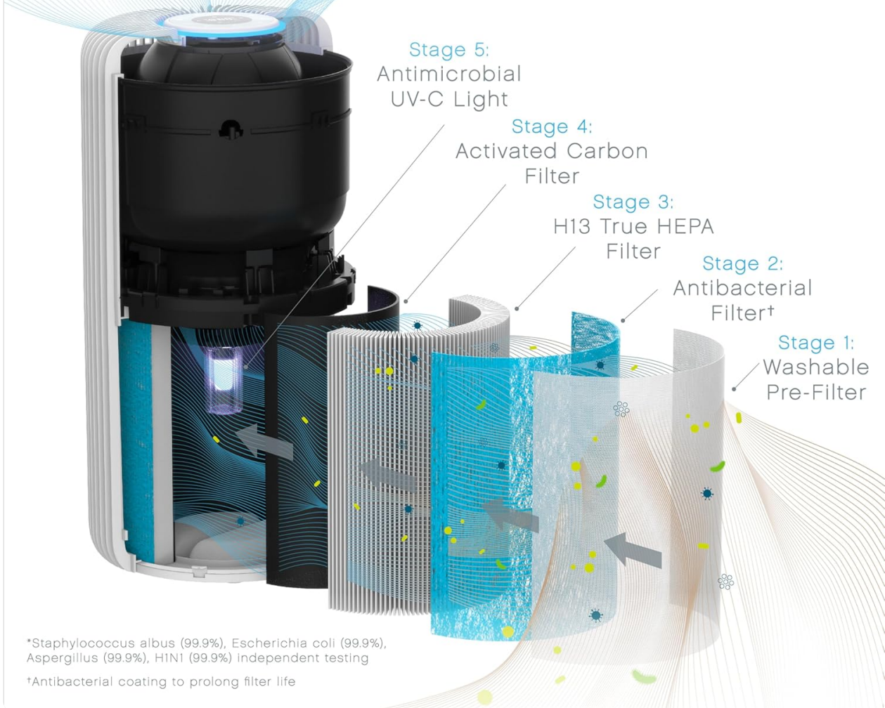
Figure 4: Detailed view of the 5-stage air purification process.
