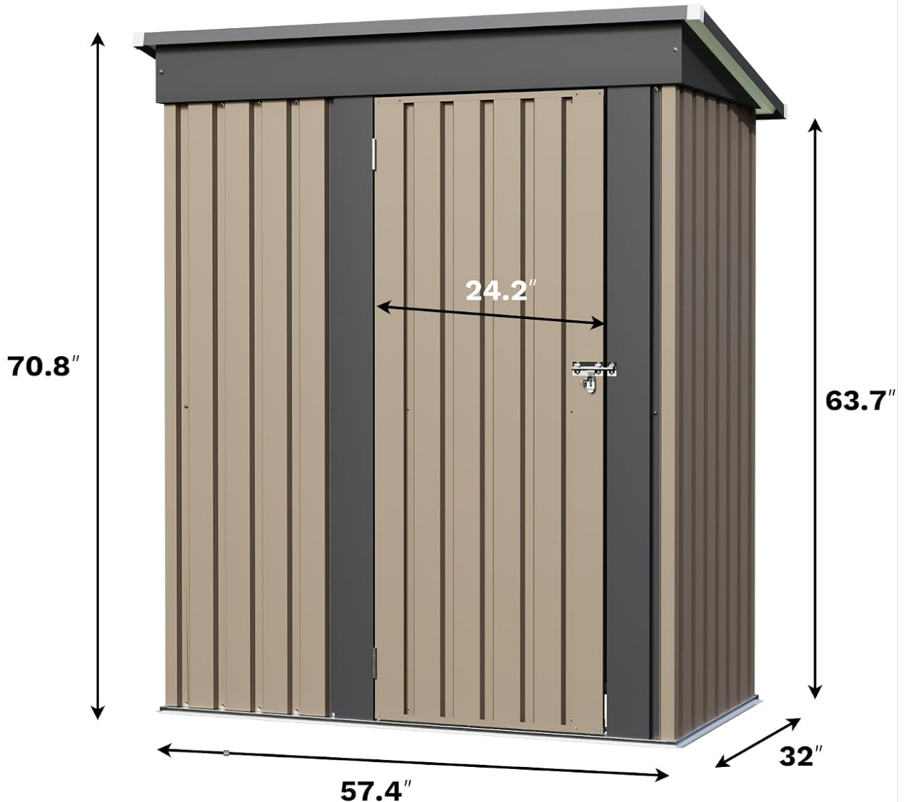
Figure 8.1: Dimensional diagram of the JUMMICO 5x3 FT storage shed, showing key measurements including height, width, and depth.
