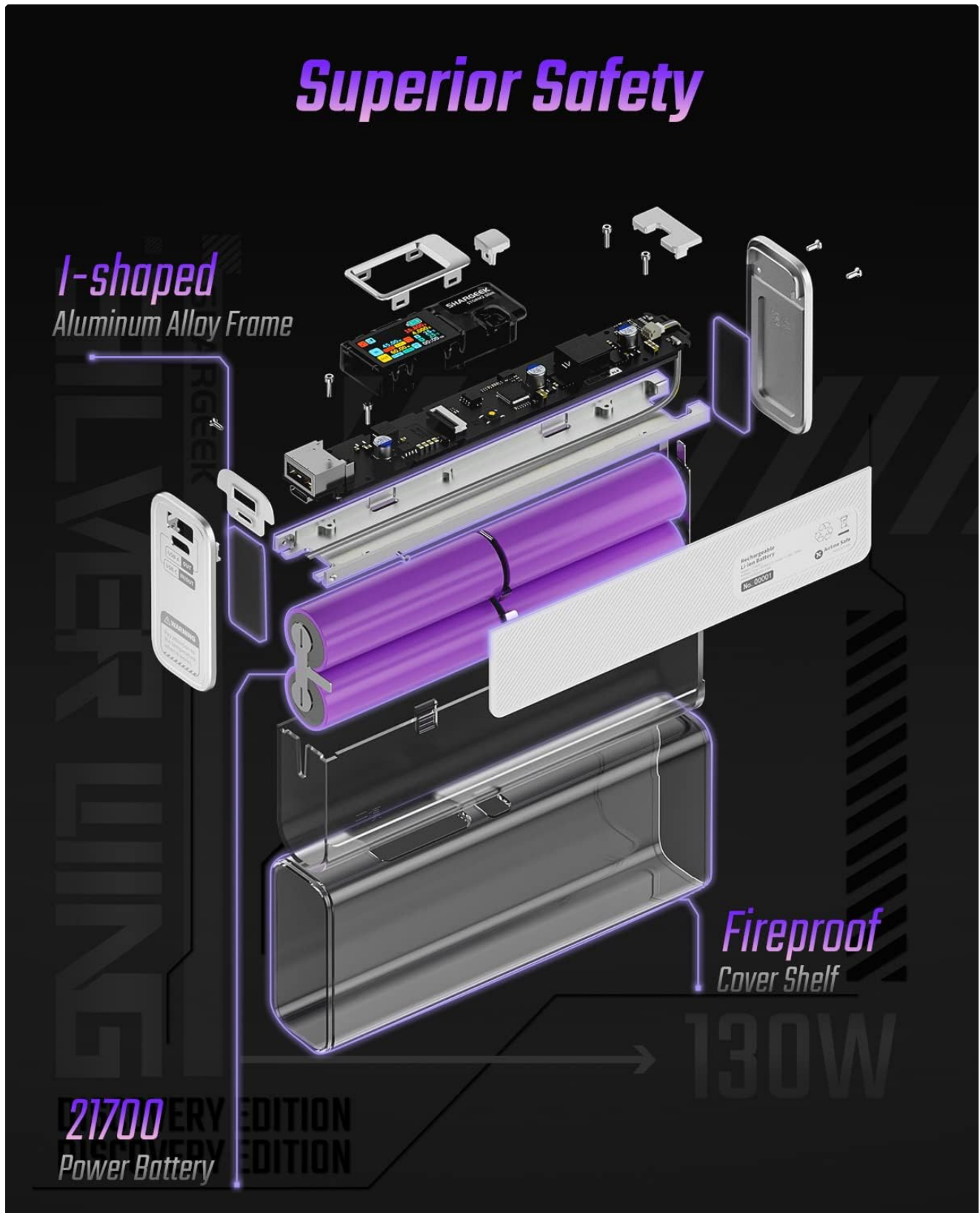
Image: An exploded diagram of the Shargeek STORM2 Slim, illustrating its internal structure including the I-shaped aluminum alloy frame, fireproof cover shelf, and 21700 power batteries, highlighting its robust construction.
