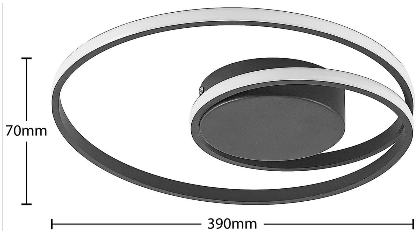
Image 4.2: Product dimensions for installation planning.
