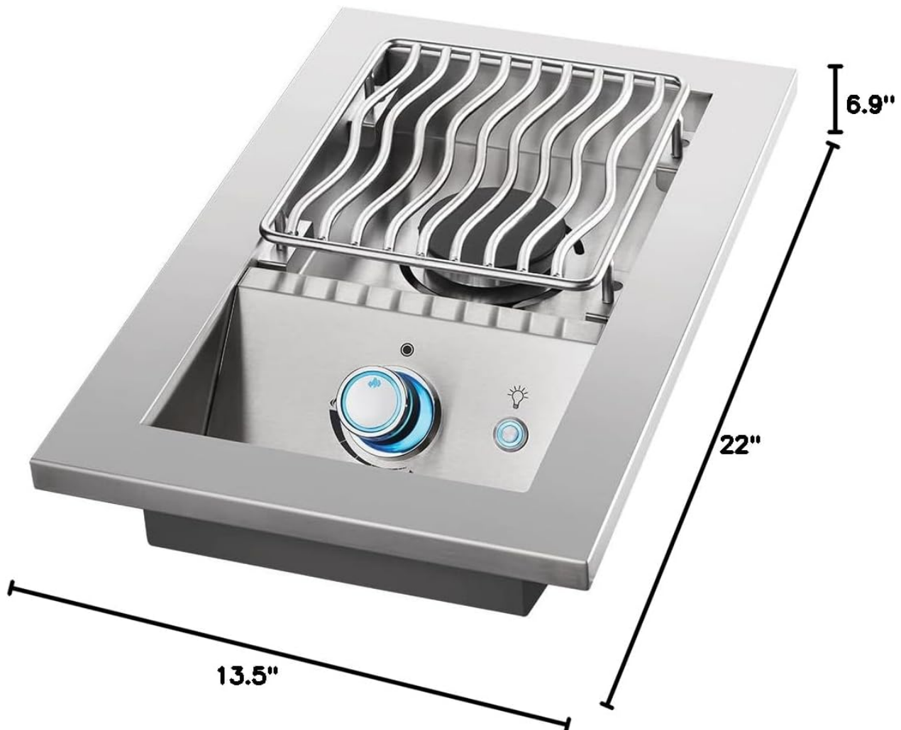
Figure 4.1: Product Dimensions (22"D x 13.5"W x 6.9"H)
