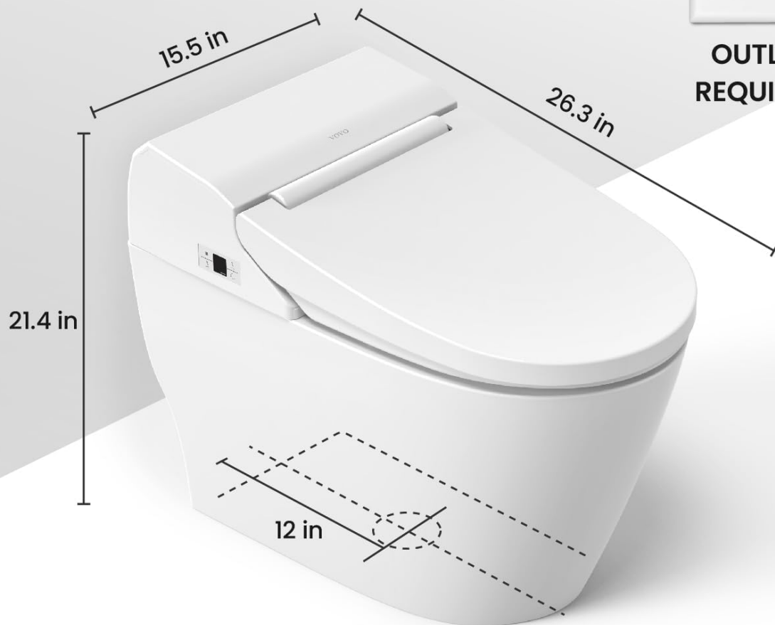
Figure 10: Important dimensions for installation and a reminder that an electrical outlet is required.
