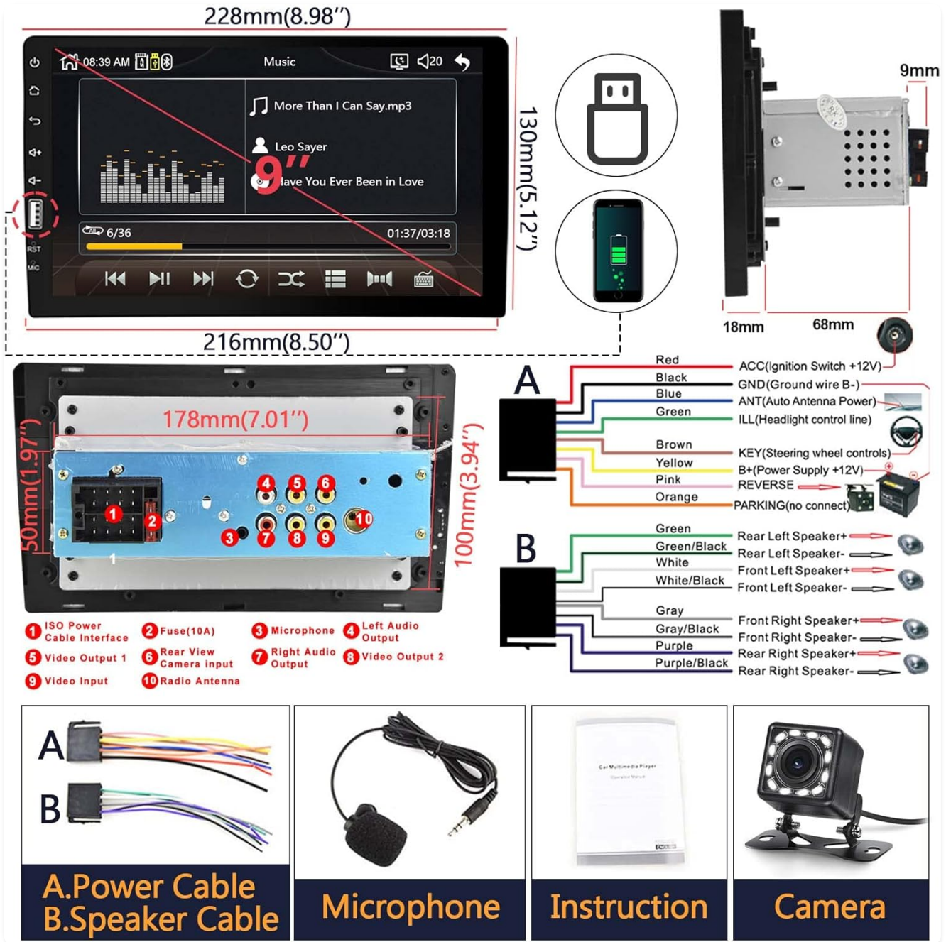
Figure 4.1: Wiring connections and dimensions for the car stereo.
