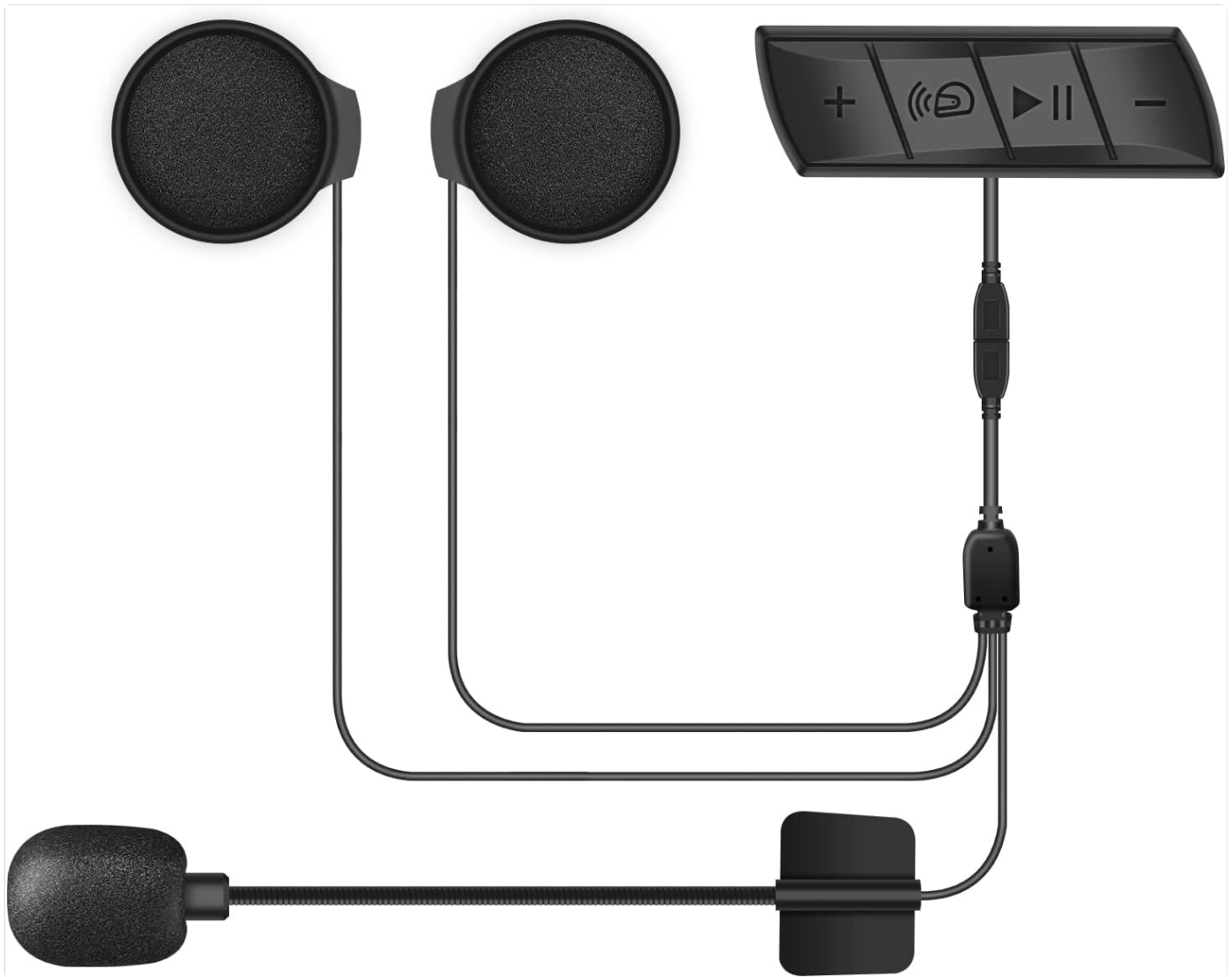
Image: Overview of the VR-robot M7 headset components, including the main control unit, speakers, and microphone.
