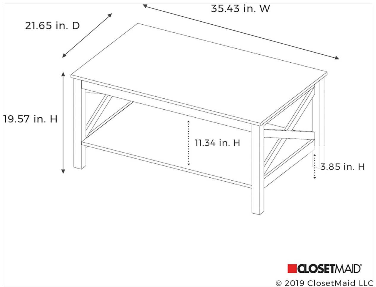
Image 4.1: Dimensional diagram of the coffee table, showing its height, width, and depth.
