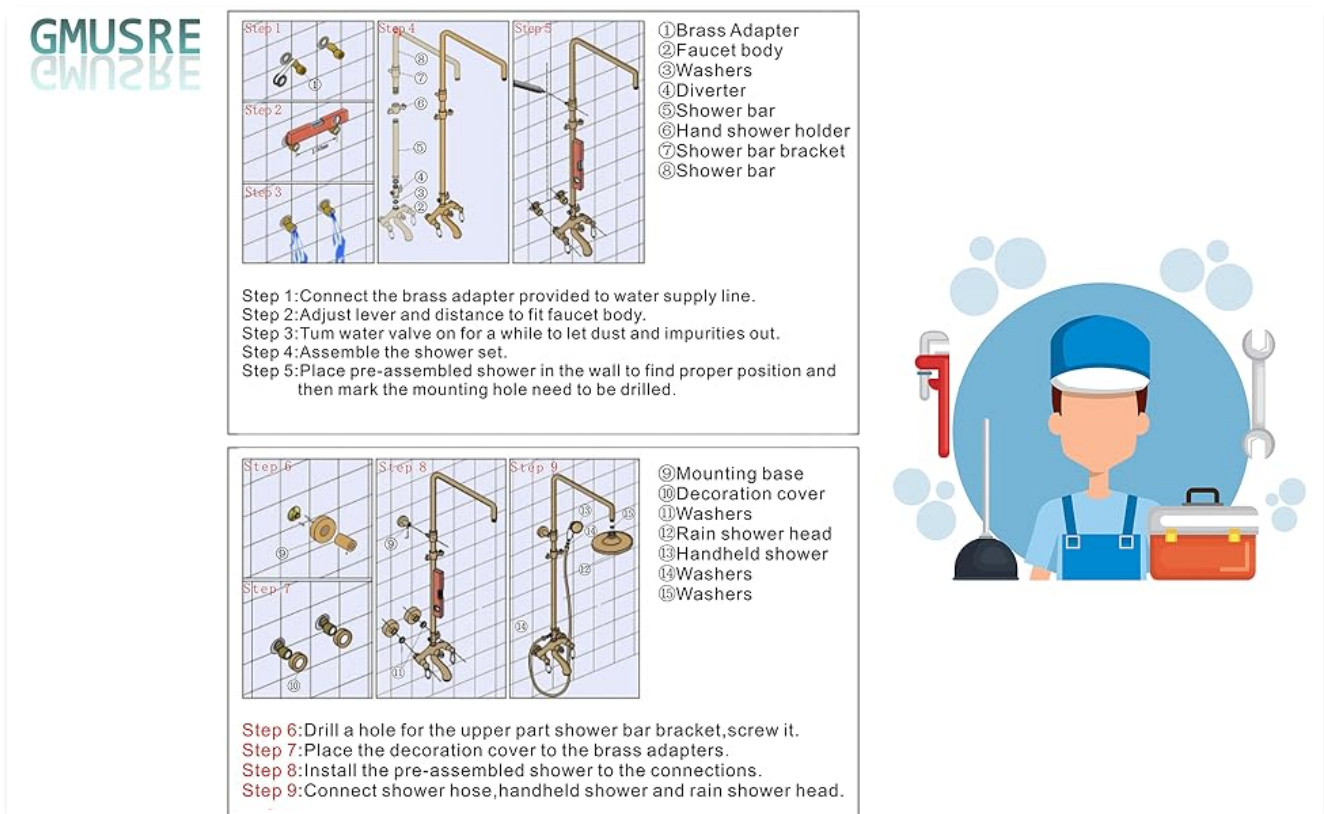
Image: Detailed diagram illustrating the installation steps and components for the Gmusre shower system.
