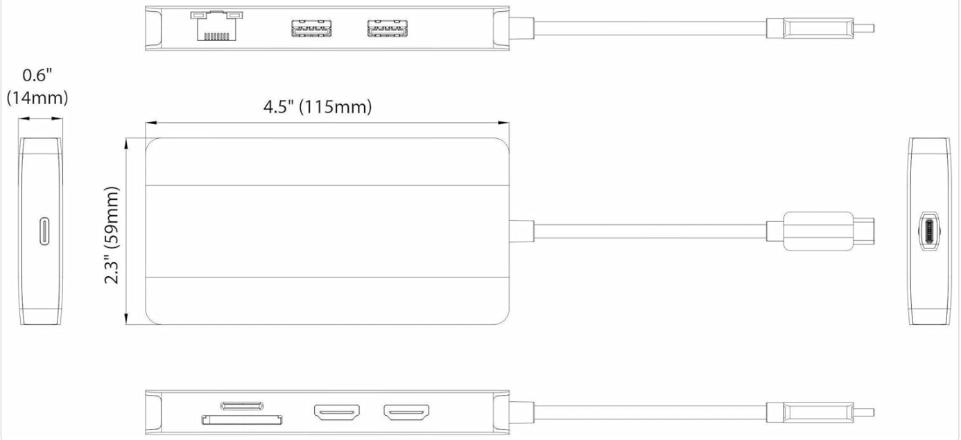
Figure 7.1: Diagram illustrating the product dimensions. The image provides measurements for the length (4.5 inches / 115mm), width (2.3 inches / 59mm), and height (0.6 inches / 14mm) of the docking station.
