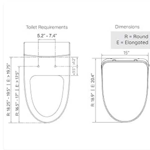
Figure 8: Product Dimensions and Toilet Requirements. This diagram provides essential measurements to ensure compatibility with your toilet.
