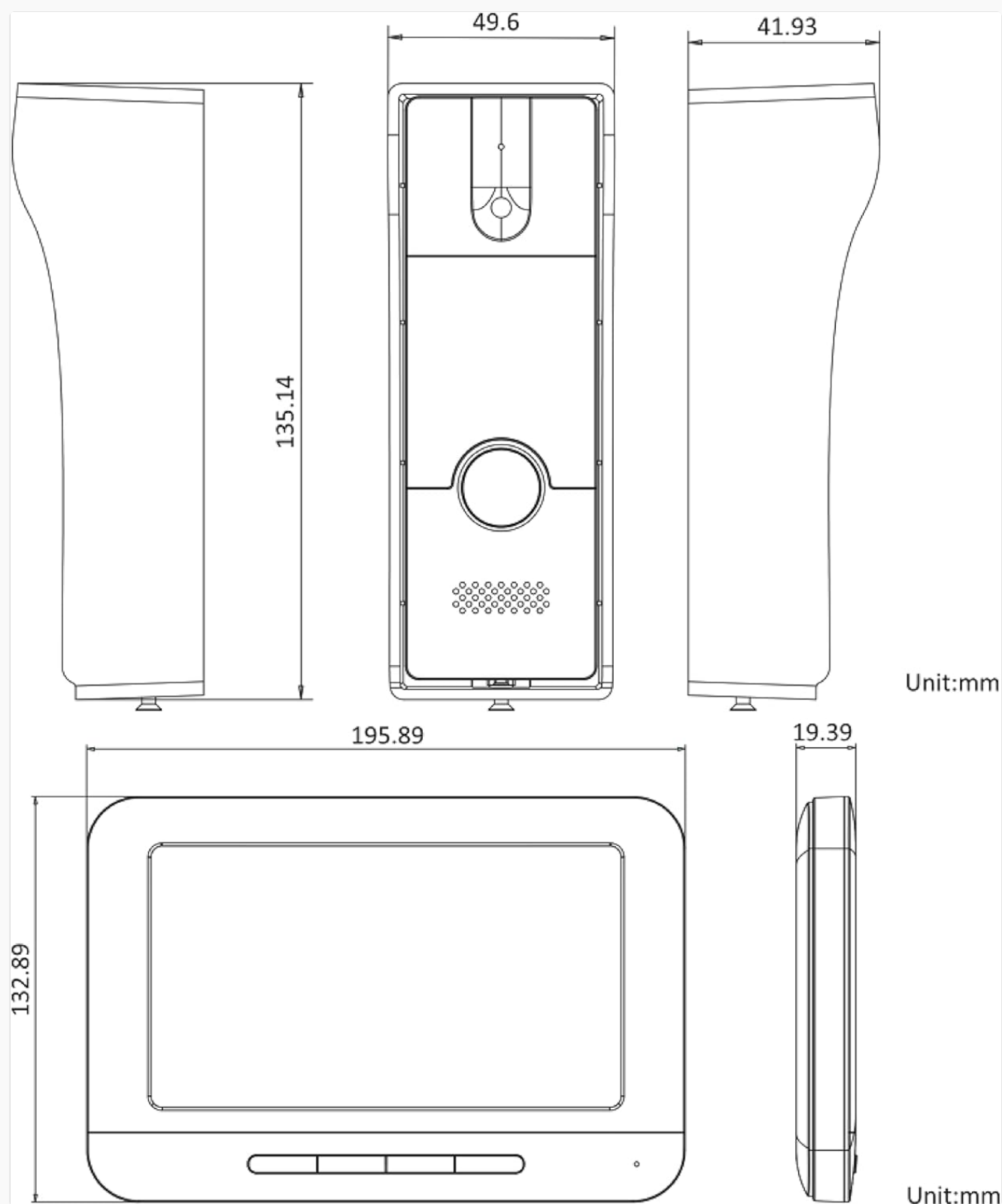
Figure 4: Detailed technical drawing showing the dimensions of both the indoor monitor and the outdoor unit of the Hikvision DS-KIS202T system.
