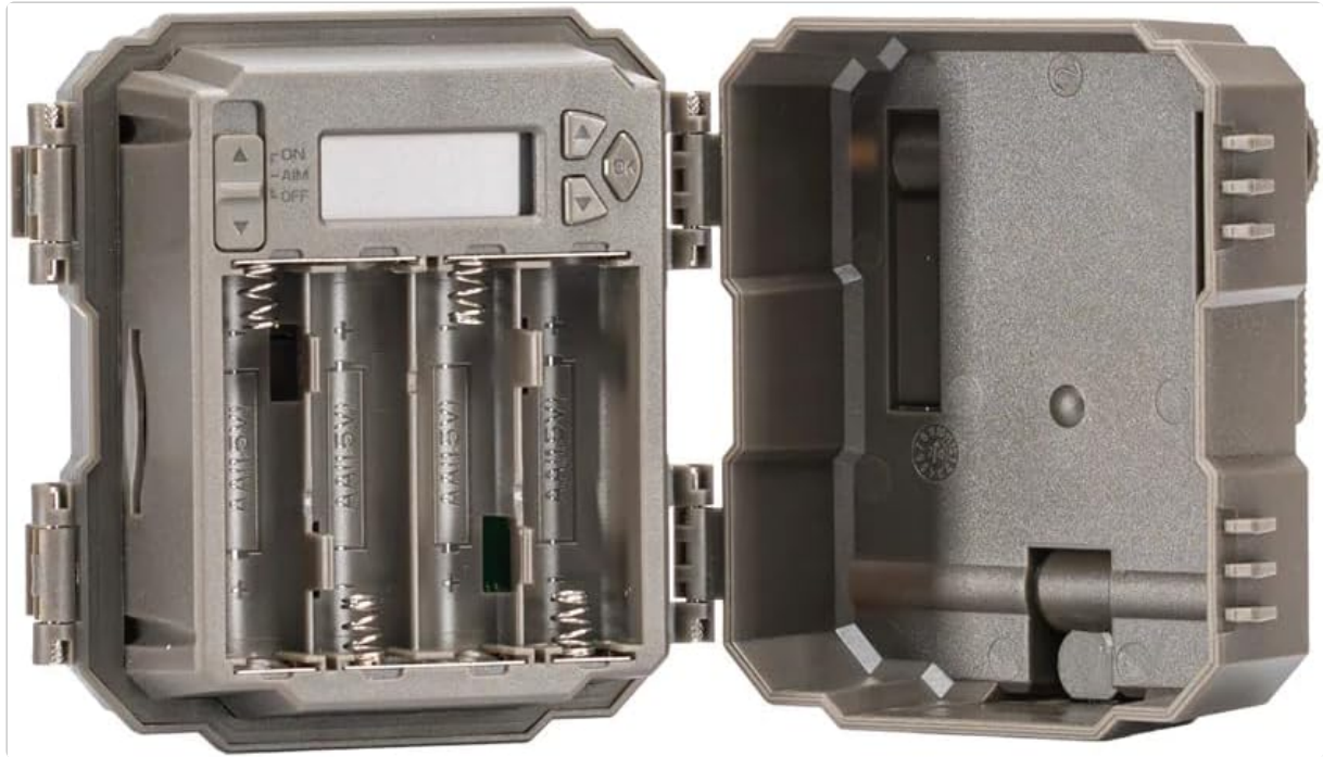
Figure 1: Open camera housing showing the battery compartment for 4 AA batteries.
