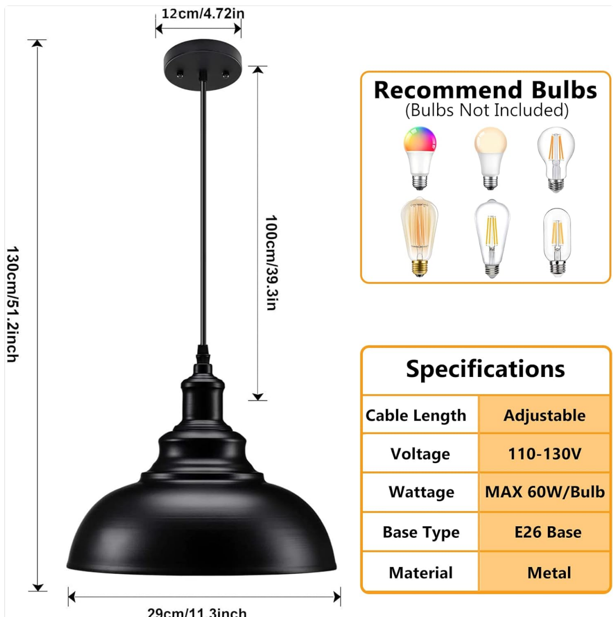
Image 4.1: Detailed dimensions of the pendant light and a summary of key specifications.
