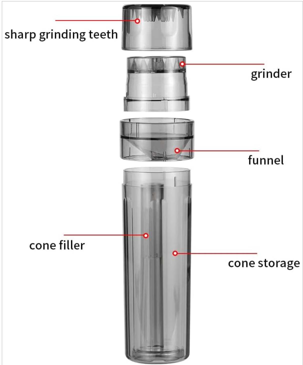
Image 3.1: An exploded diagram illustrating the various parts of the JOUGE grinder, including the grinding teeth, funnel, cone filler, and storage compartment.
