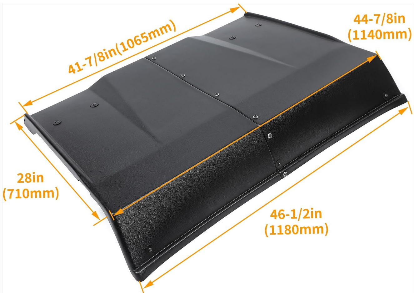
Image 4.1: Product dimensions for reference.
