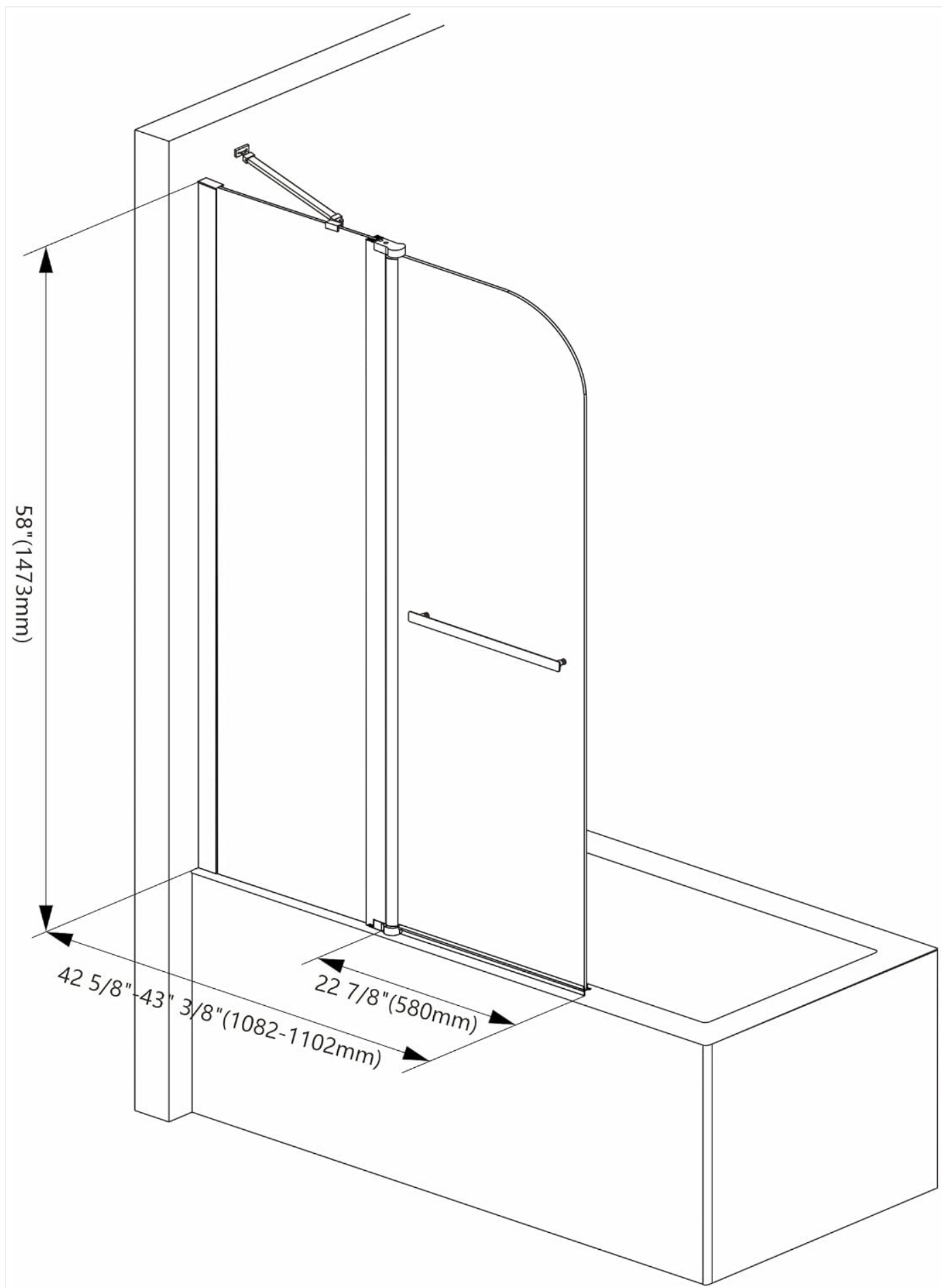
Image: Dimensional diagram for the Sunrosa Pivot Tub Shower Door.
