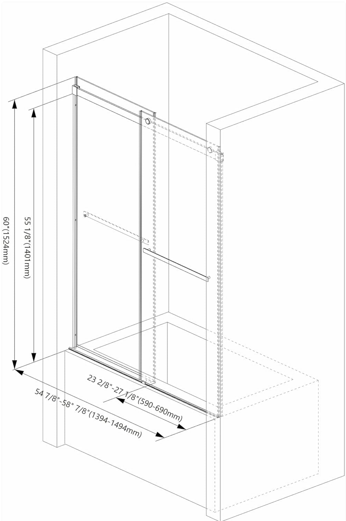
Figure 4: Dimensional drawing of the shower door, indicating adjustable width and height. Ensure your space accommodates these measurements.
