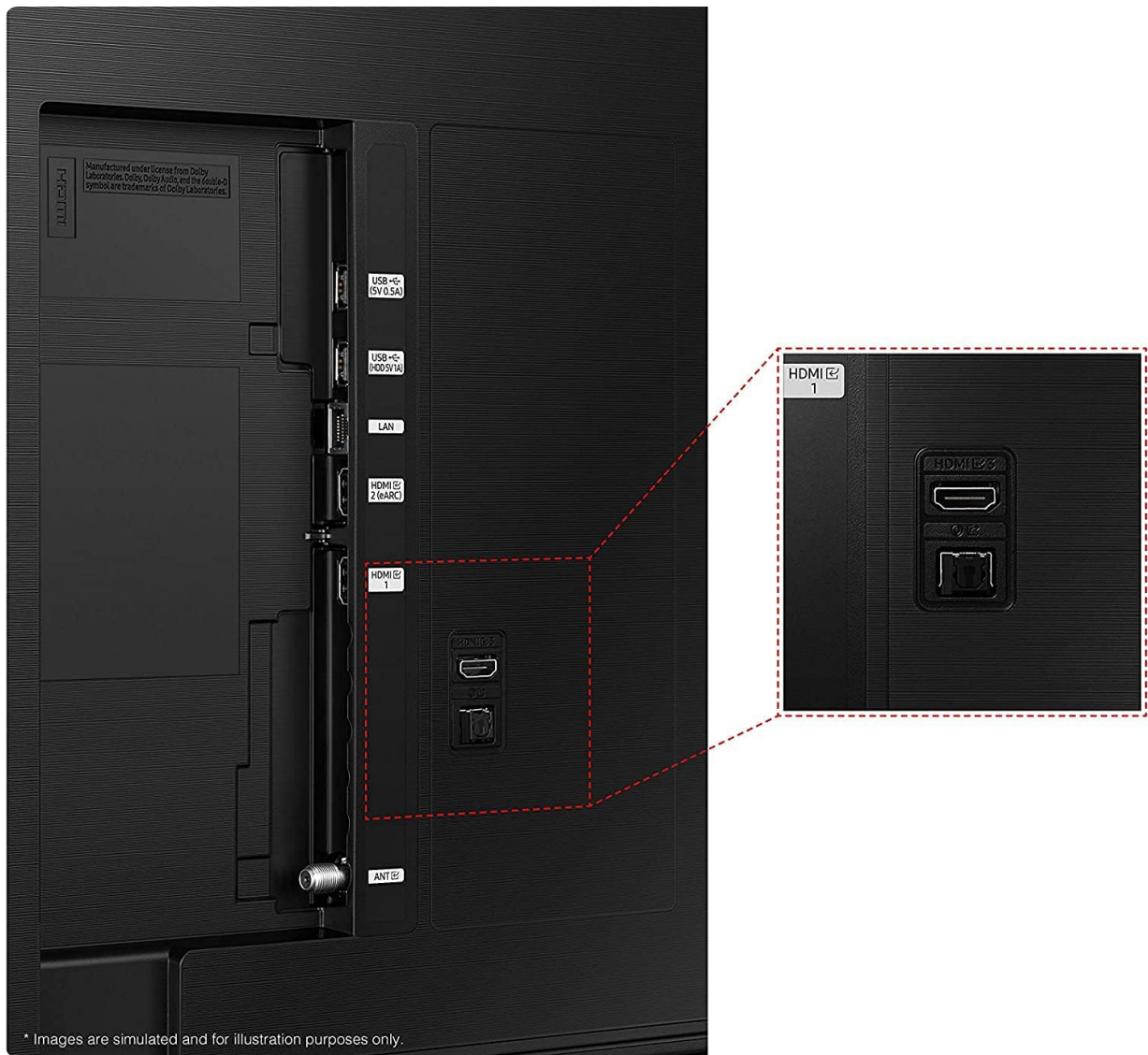
Image: A detailed view of the back of the Samsung QLED TV, highlighting the HDMI, USB, LAN, and other connectivity ports for external devices.
