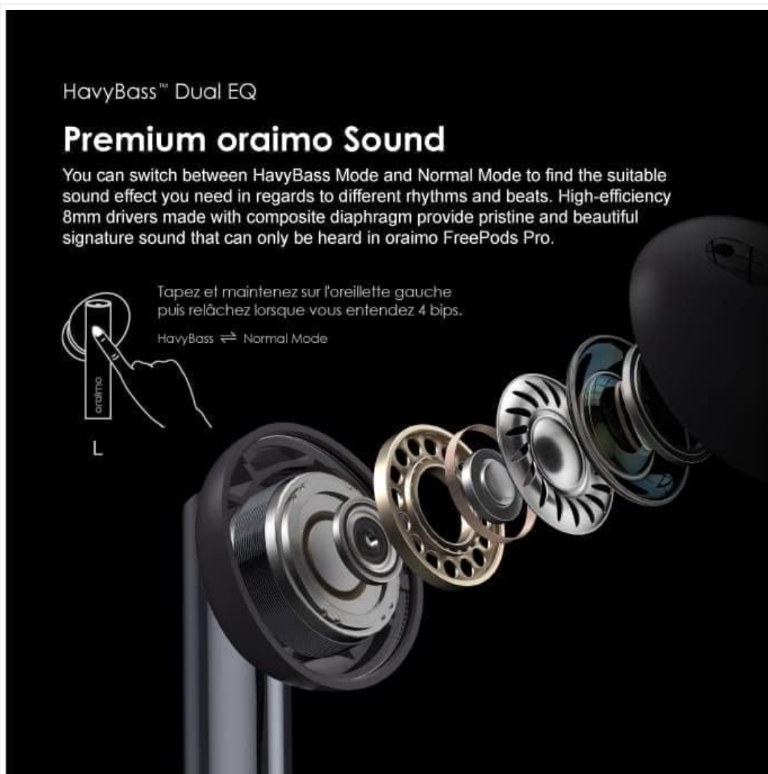
Image: Exploded view of an earbud showing internal components and a diagram illustrating the tap gesture on the left earbud to switch between HavyBass and Normal sound modes.
