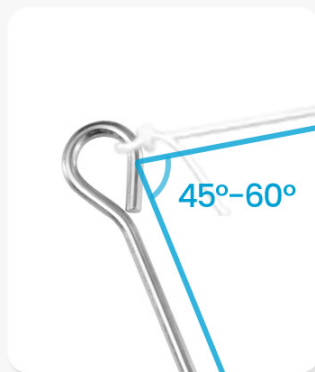
Solid Metal Ground Anchors
