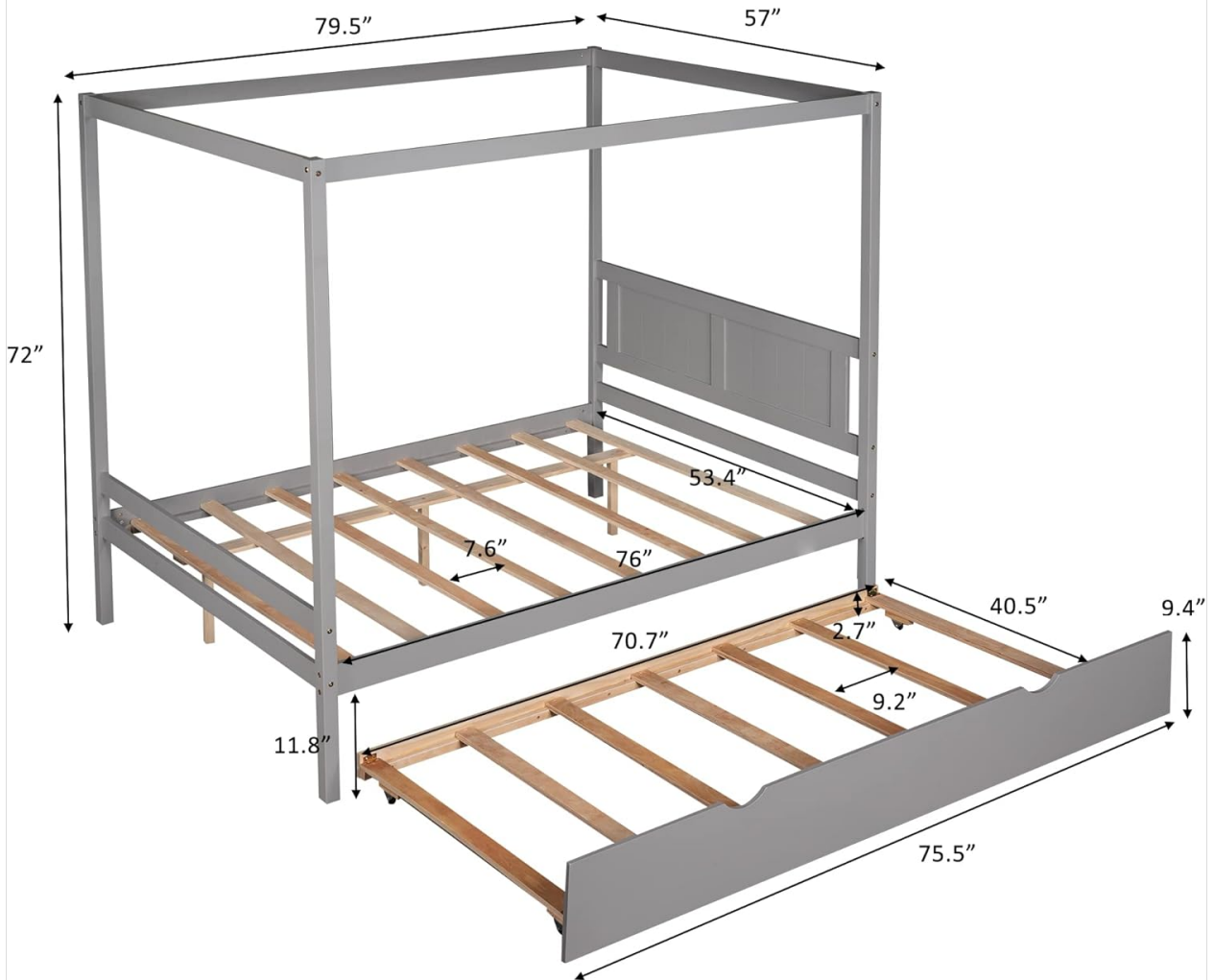
Image 8.1: Technical drawing displaying all key dimensions of the bed frame and trundle unit, including length, width, and height measurements.
