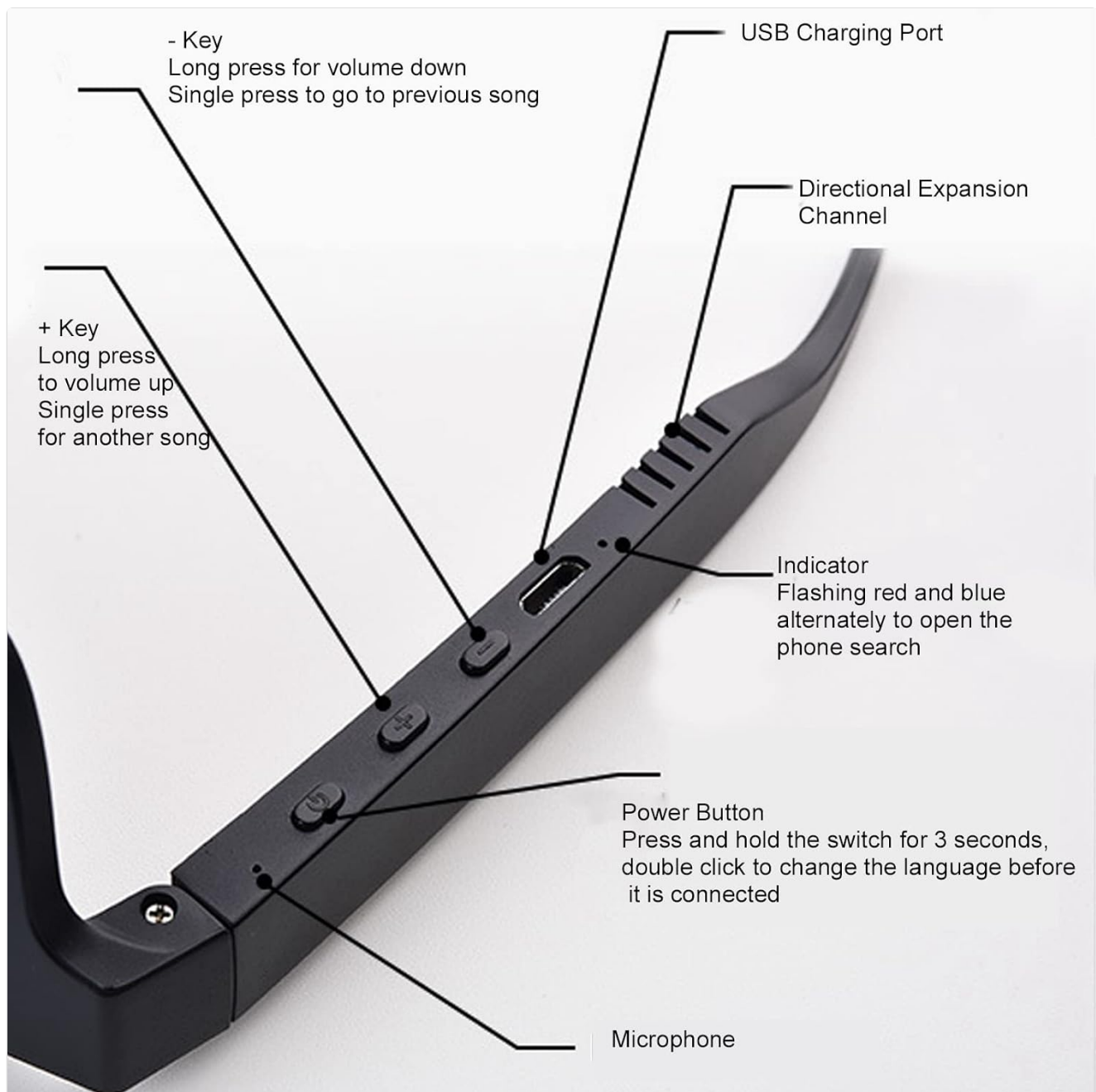
Image: Detailed diagram of the smart sunglasses' controls and features.
