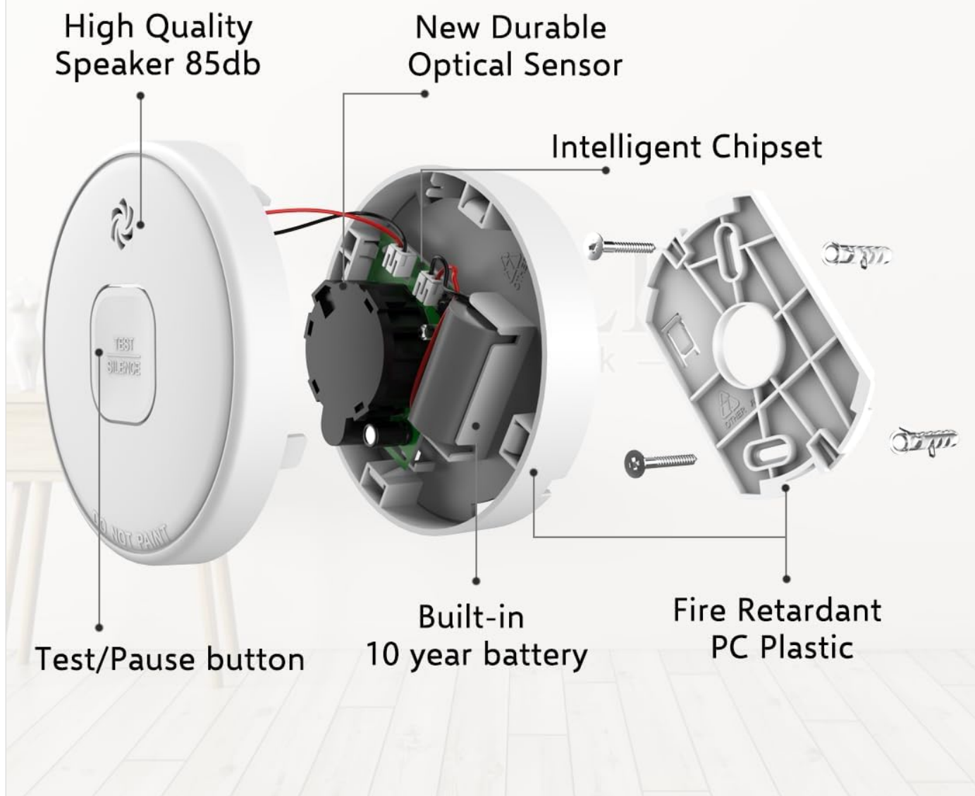
Image: Internal components and construction details of the ELRO FS2010.
