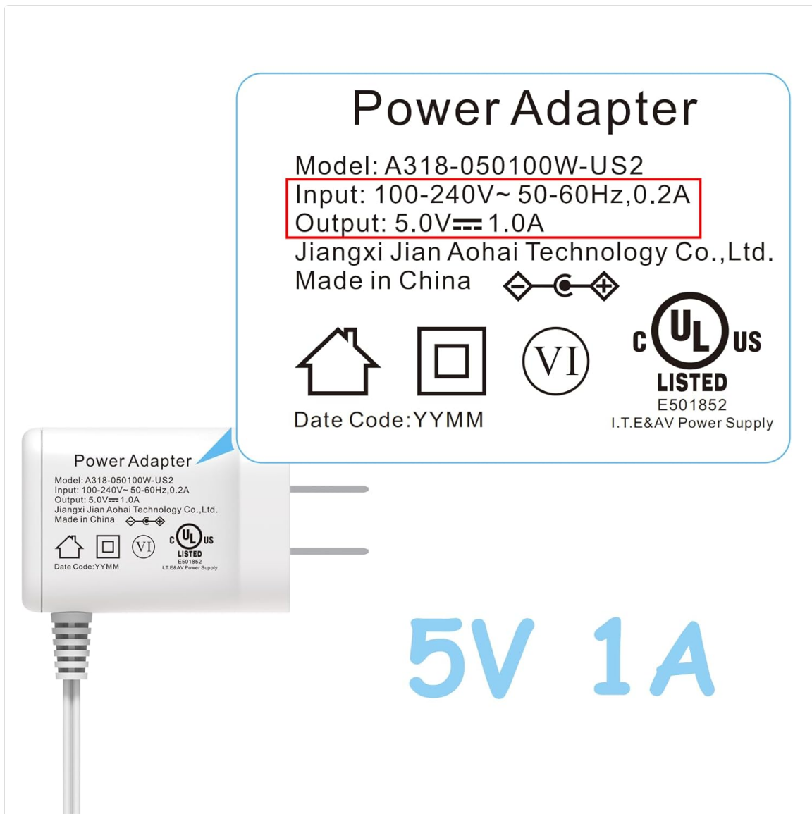
Figure 2: Power adapter details, confirming 5V 1A output for safe charging.
