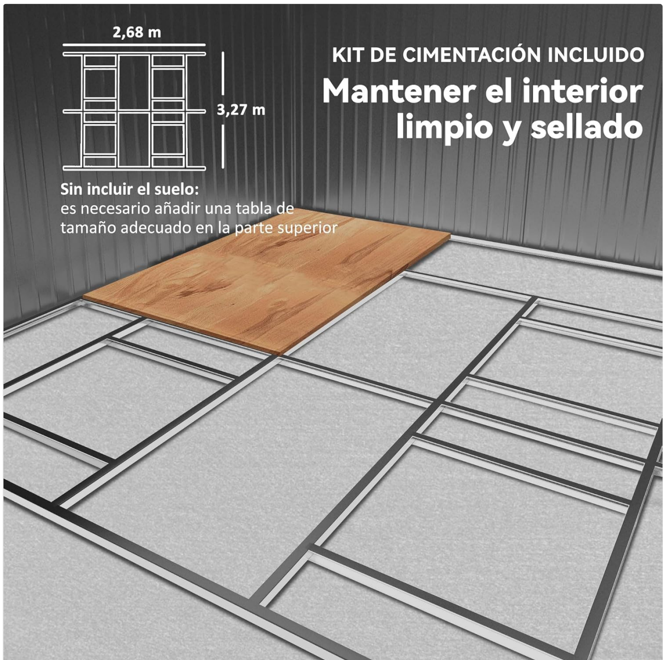
Image 5.1: A diagram showing the included foundation kit, designed to support your chosen flooring and keep the interior clean and sealed.
