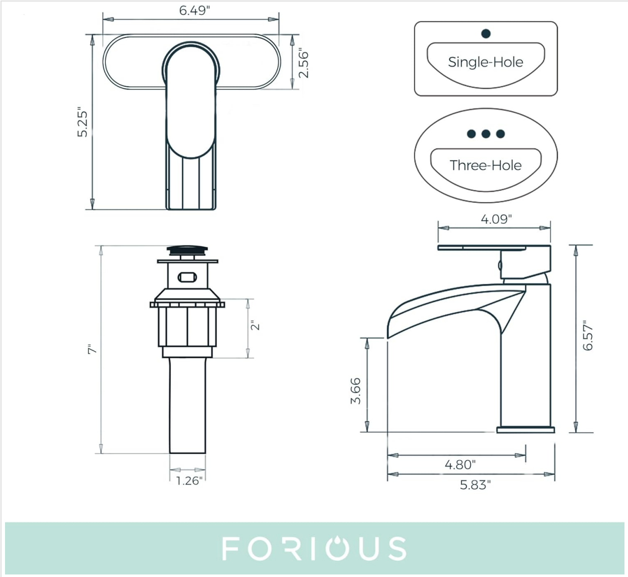
Image 4.1: Detailed dimensions of the faucet and pop-up drain.
