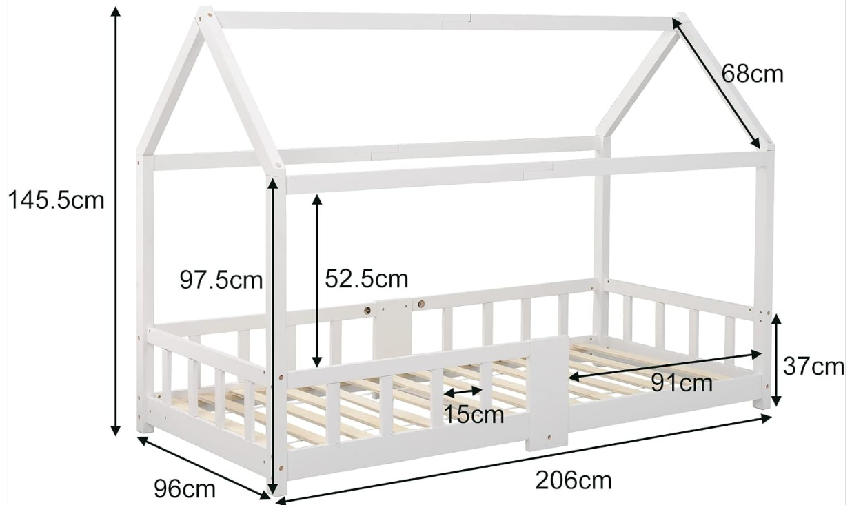
Image 4.1: Detailed Dimensions of the Bed
