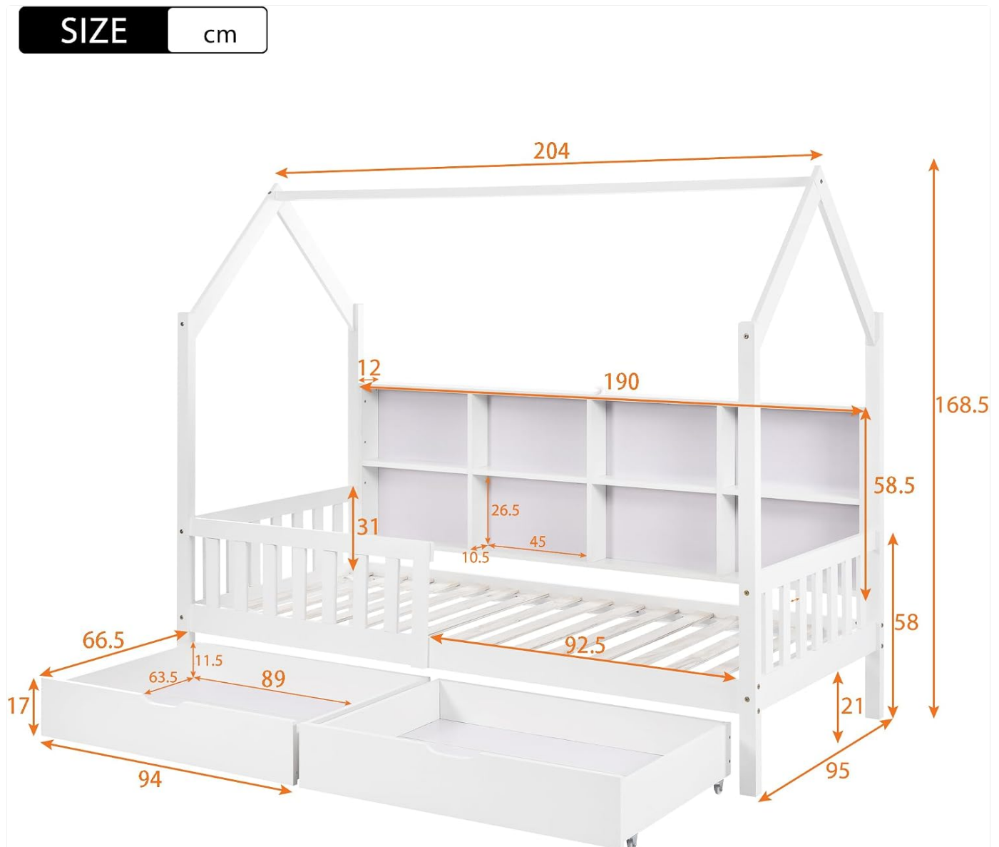
Figure 3.1: Detailed dimensions of the Moimhear Kids Bed, including overall length (204 cm), width (95 cm), height (168.5 cm), and drawer dimensions.
