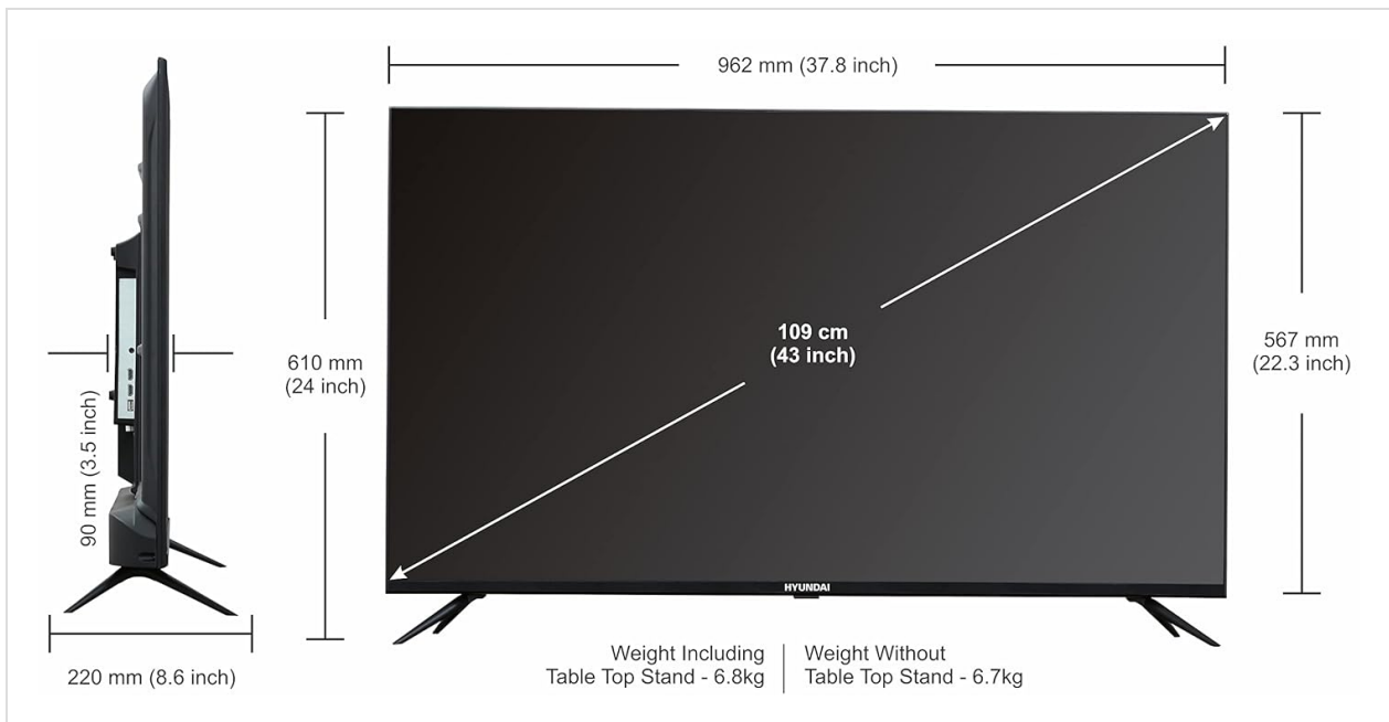
Image: Diagram illustrating the dimensions of the Hyundai 43-inch Smart LED TV, showing width, height, and depth with stand. Also indicates screen size and weights.
