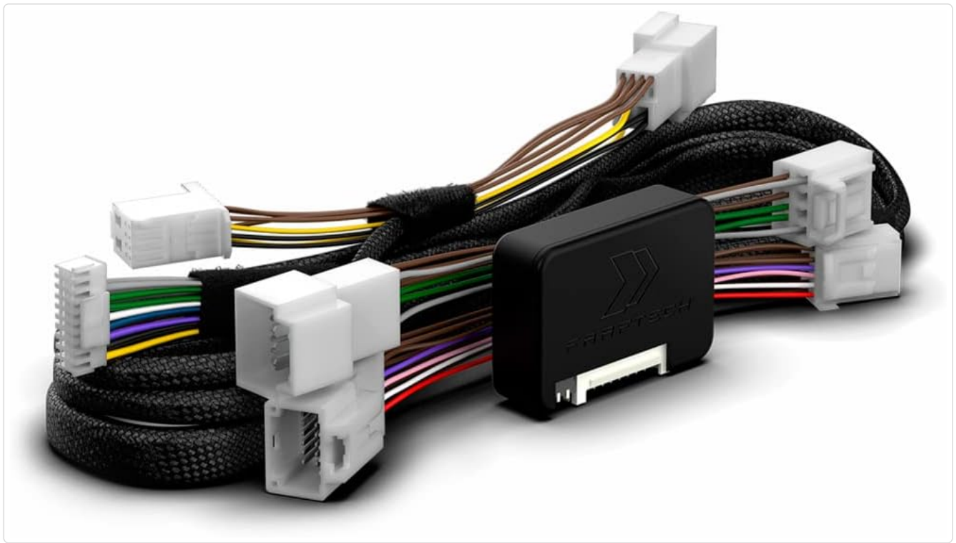
Image 2.2: A detailed view of the Faaftech FT-AC-TY3 module and its accompanying wiring harness. The harness features multiple connectors designed for seamless integration with the vehicle's electrical system.
