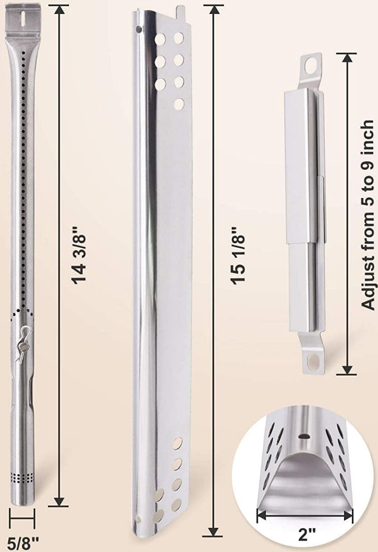
Figure 2: Product dimensions for burner tubes, heat plates, and crossover tubes.
