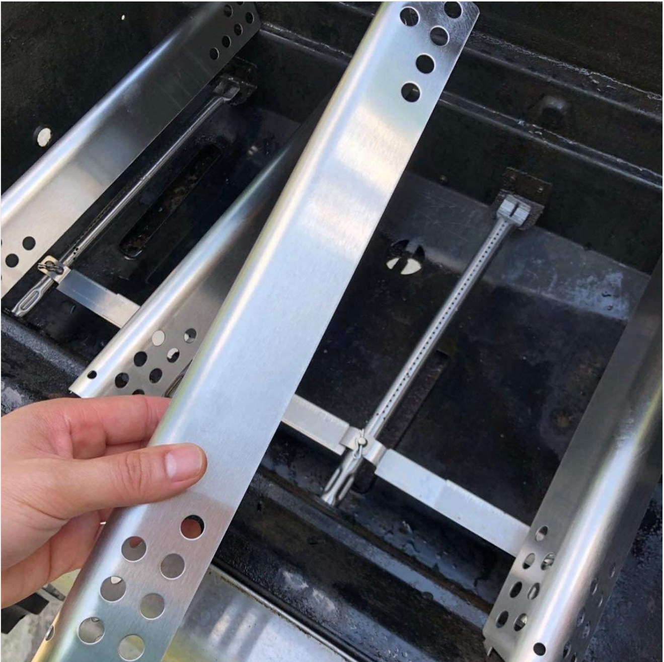
Figure 5: Installing a new heat plate into the grill.
