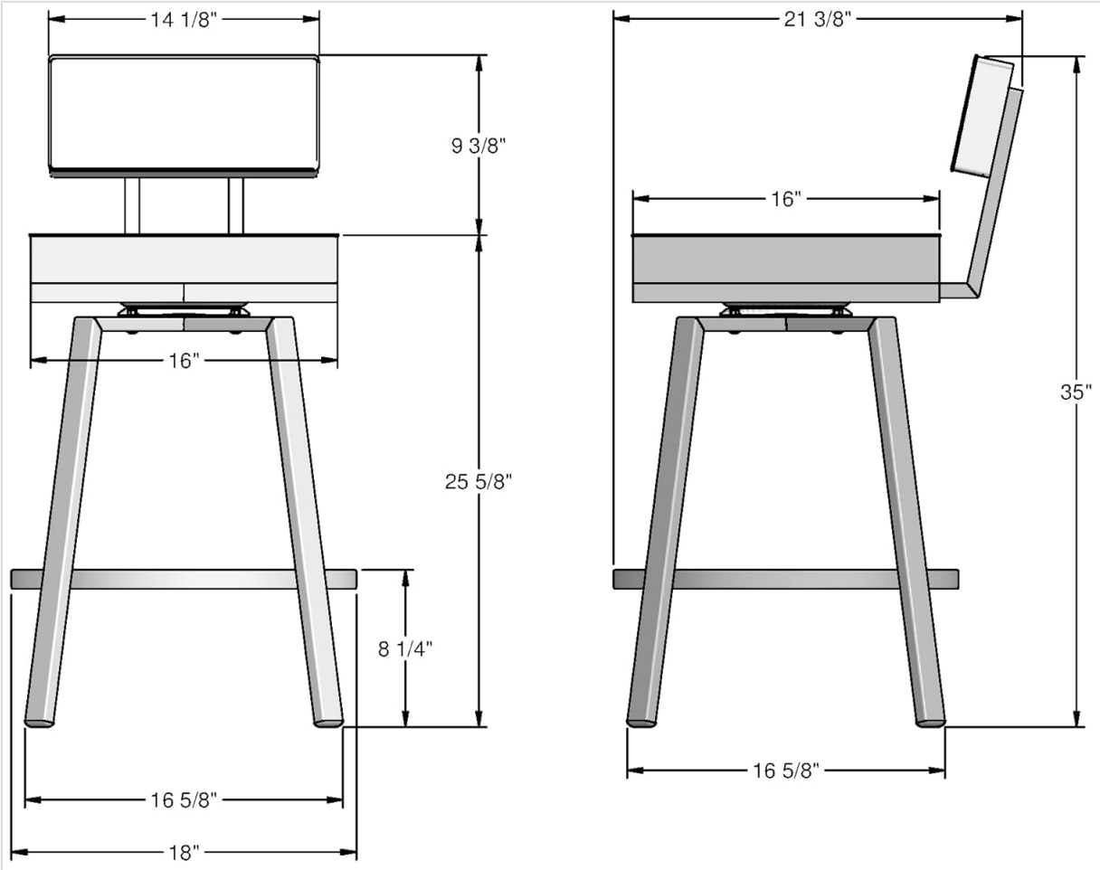
Image: Technical drawing illustrating the dimensions of the Amisco Staten Counter Stool.
