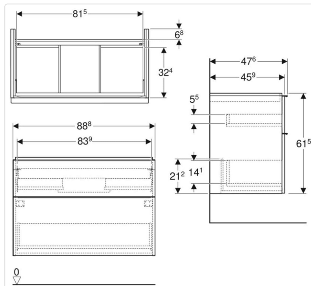
Figure 2: Technical drawing illustrating the dimensions of the Geberit iCon washbasin cabinet. Key measurements include a width of 888mm, a height of 615mm, and a depth of 476mm. This diagram is crucial for accurate installation planning.
