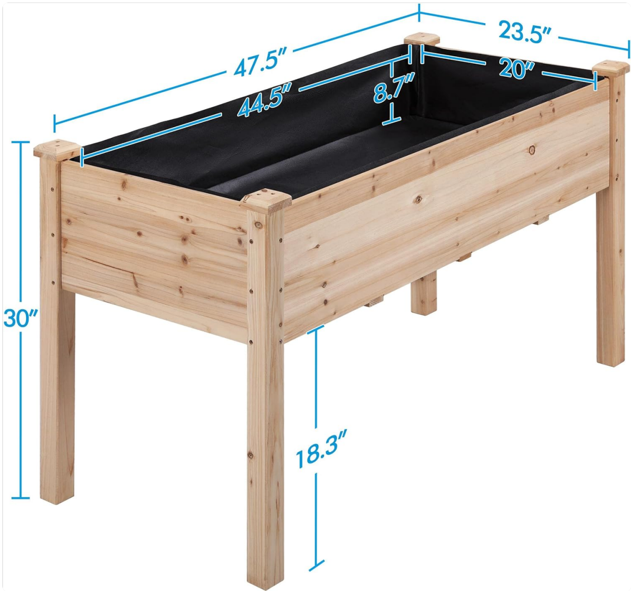
Image: Product dimensions.
