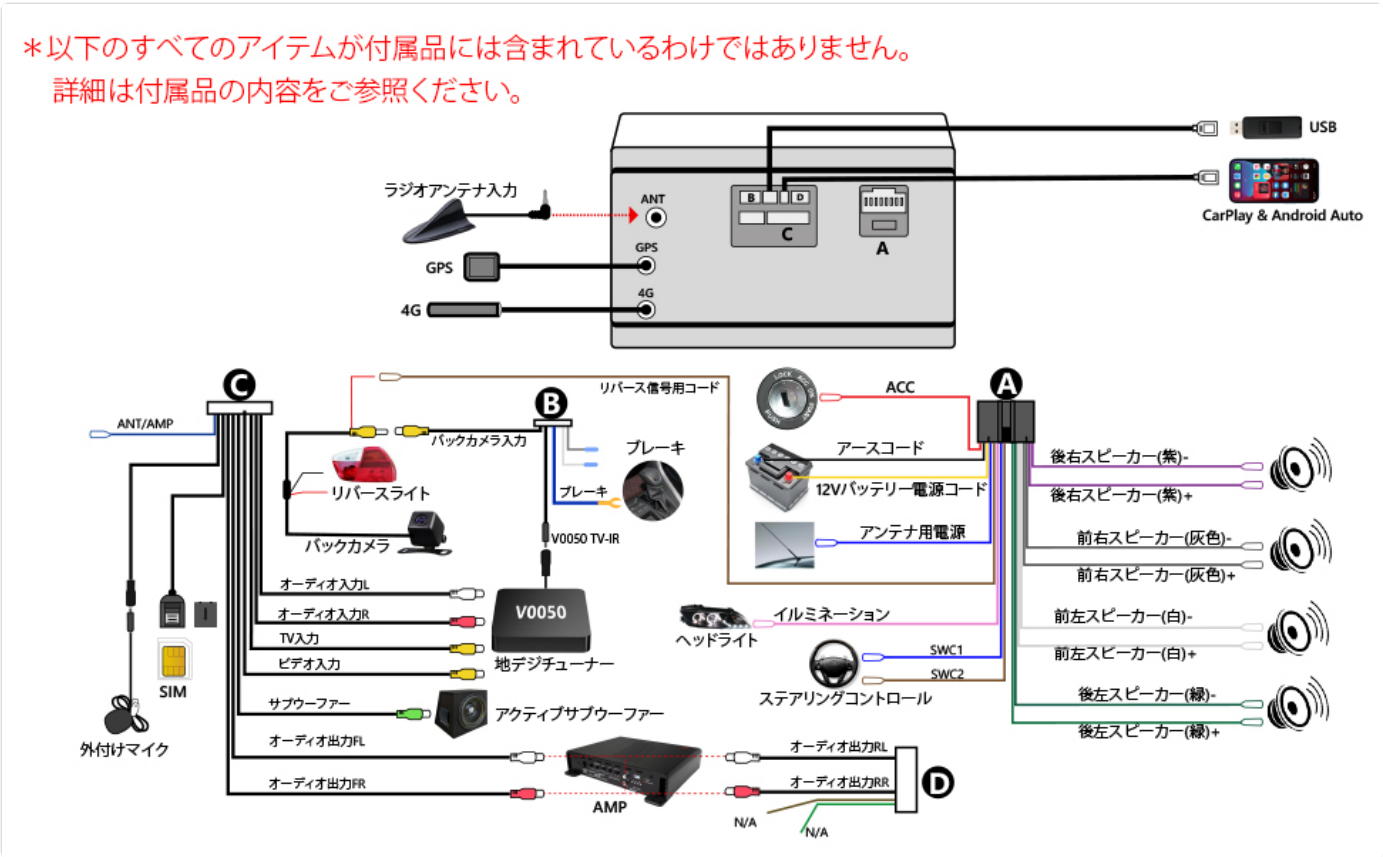
Figure 3.2: Wiring Diagram. This diagram illustrates the connections for power, speakers, GPS, 4G, USB, CarPlay/Android Auto, reverse light, brake, illumination, steering wheel control, and various optional accessories.
