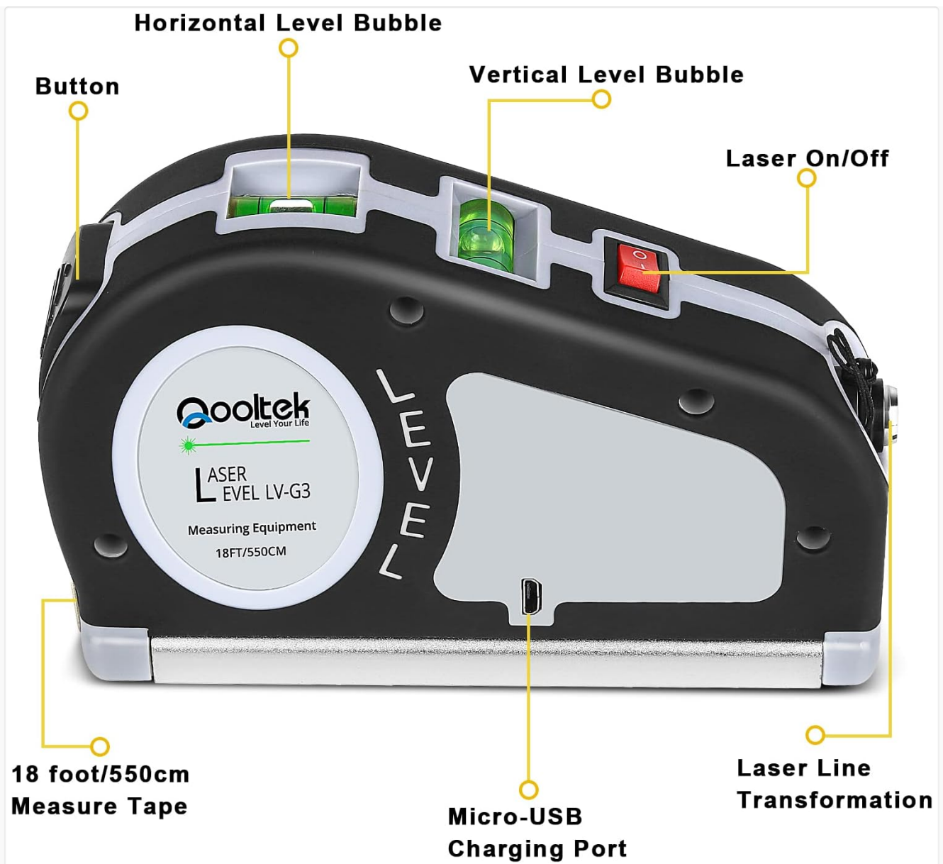
Figure 2: Labeled components of the Qooltek LVG3, including Horizontal Level Bubble, Vertical Level Bubble, Laser On/Off switch, Laser Line Transformation button, Micro-USB Charging Port, and 18ft/5.5m Measure Tape.
