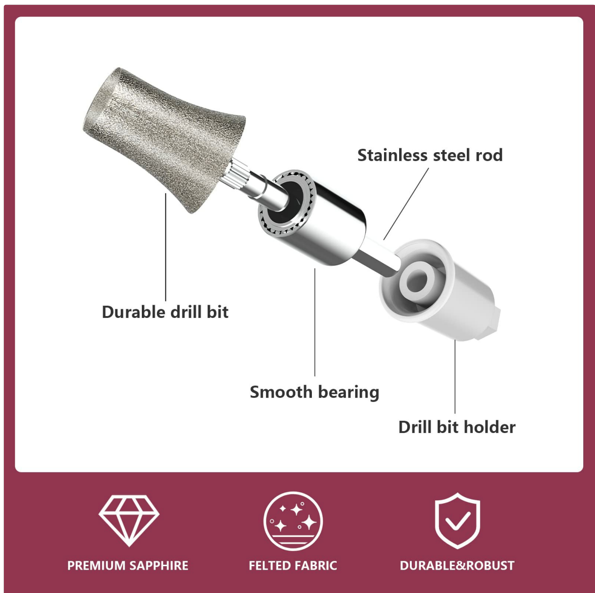
Image 3.1: Exploded view of the Sapphire Callus Sander bit. This diagram illustrates the internal components, including the durable drill bit, smooth bearing, stainless steel rod, and drill bit holder, highlighting its robust construction.
