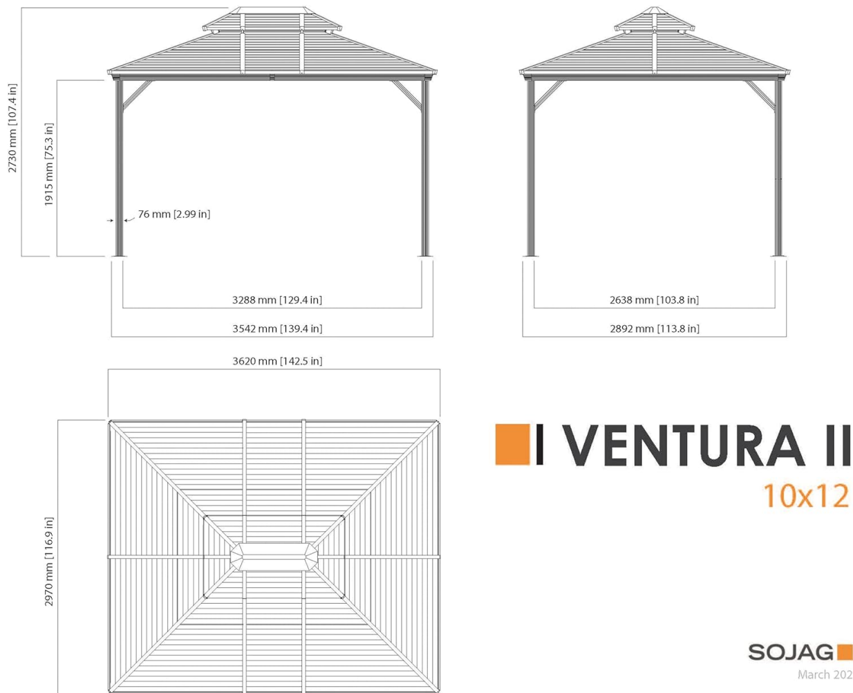
Image 4.1: Technical drawing illustrating the dimensions and structure of the gazebo.
