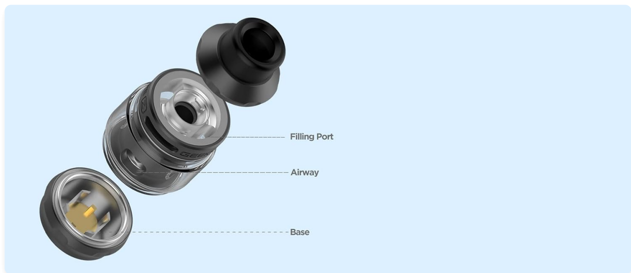
Image 2.1: Exploded diagram of the Z Sub-Ohm Tank components.
