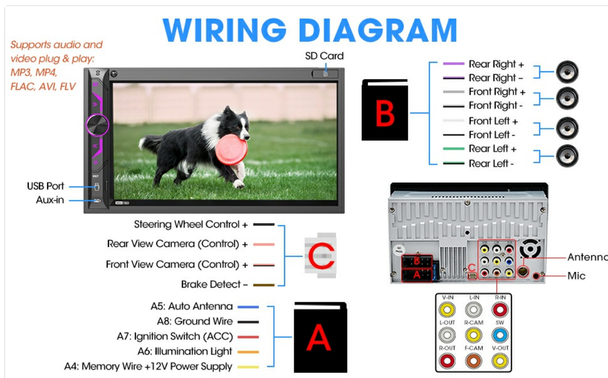
Image 4.1: Detailed wiring diagram showing connections for power, speakers, USB, AUX-in, steering wheel control, and camera inputs.
