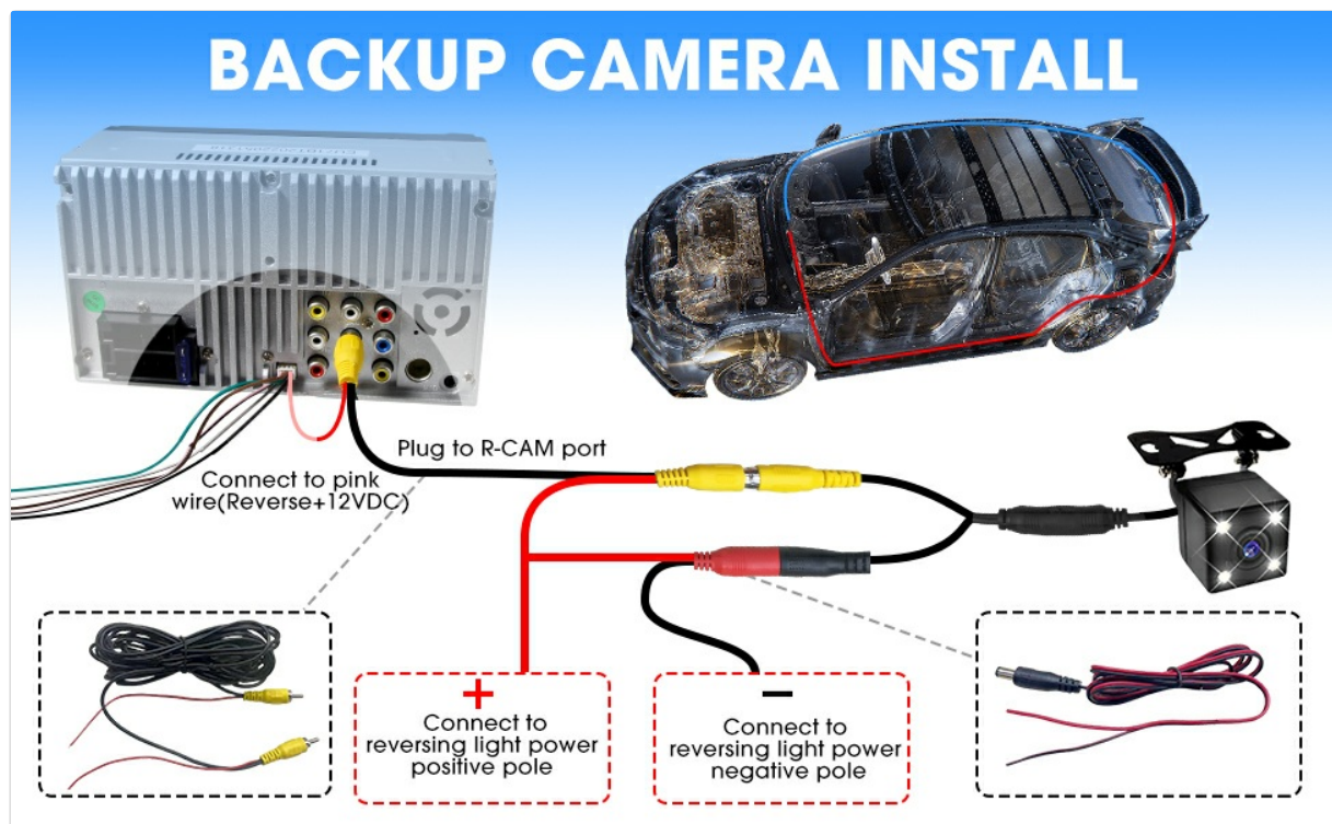
Image 4.2: Visual guide for connecting the backup camera to the car stereo and vehicle's reversing light system.
