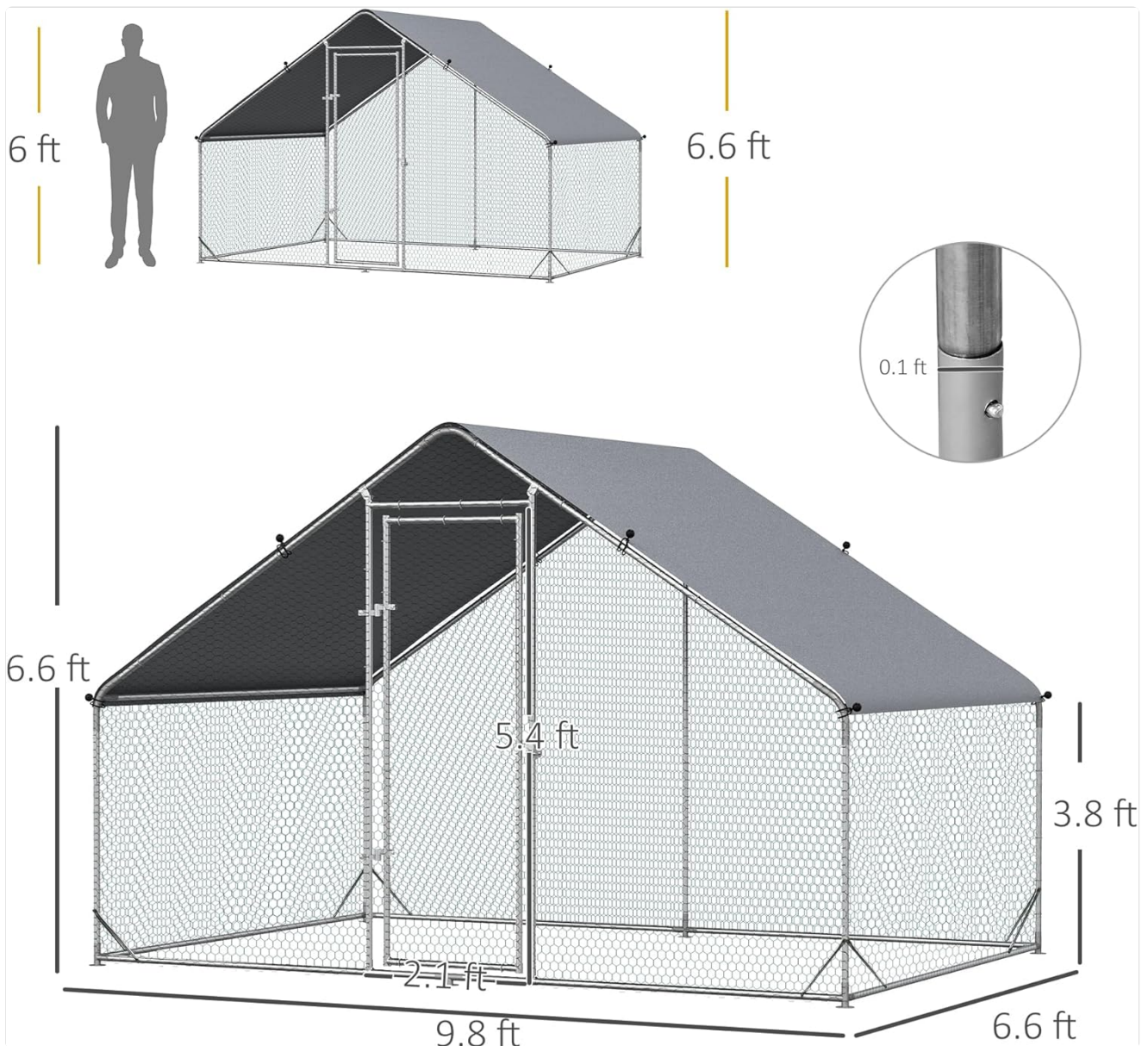
Image: Dimensions Diagram - Illustrates the overall dimensions of the coop.
