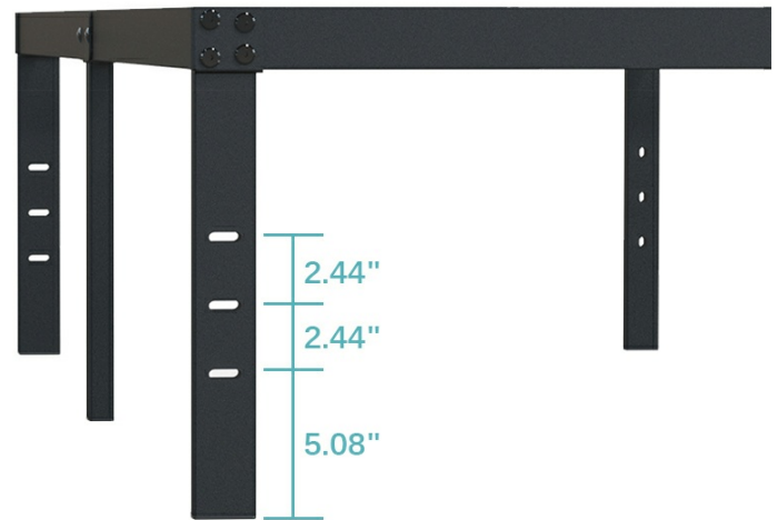
Image 4.2: The bed frame legs include three pre-drilled holes for optional headboard and footboard attachment.
